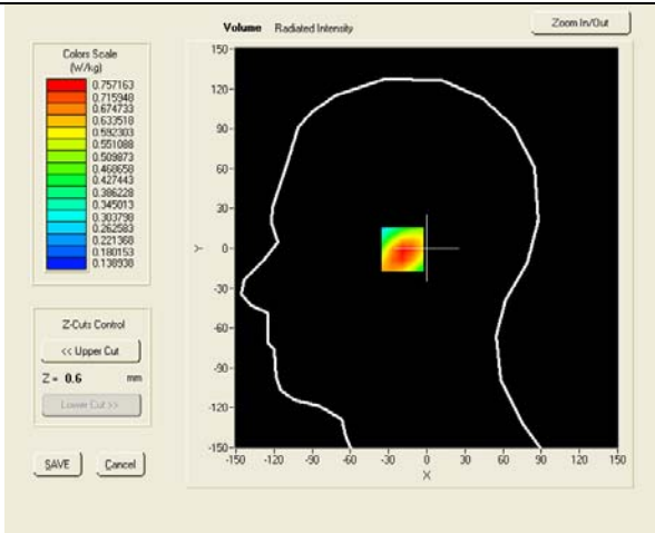
SAR, Z Axis Scan (X = -16, Y = -1)
