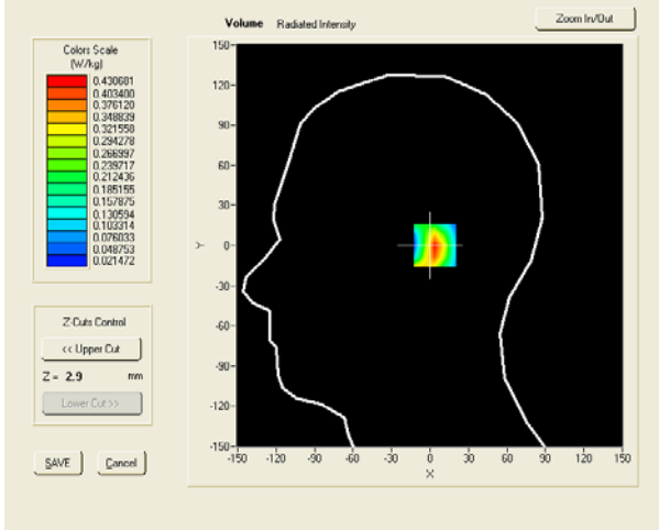
SAR, Z Axis Scan (X = 9, Y = 0)
