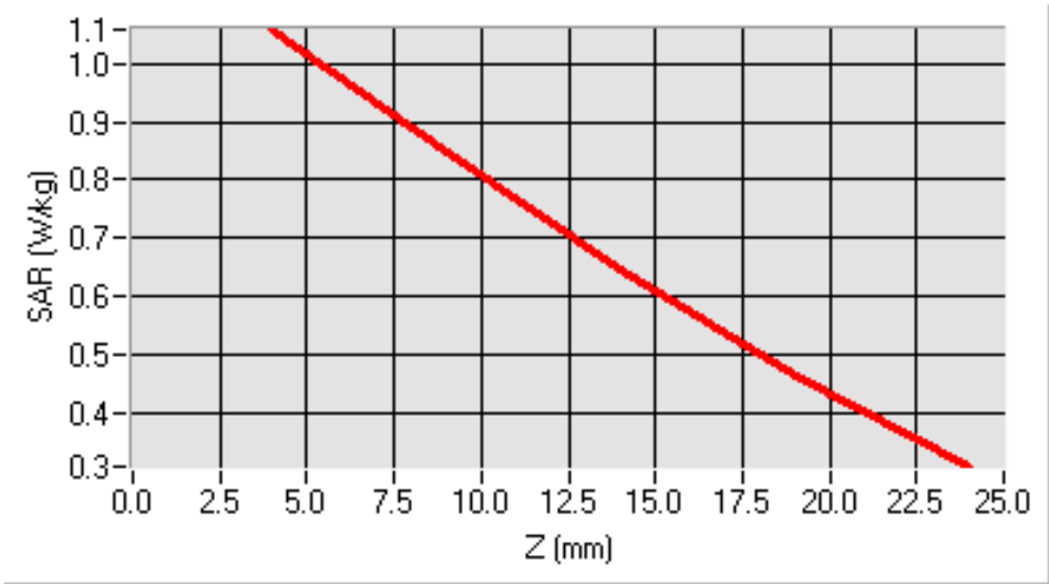
SAR, Z Axis Scan (X = -24, Y = -12)
