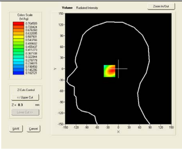
SAR, Z Axis Scan (X = -22, Y = -6)
