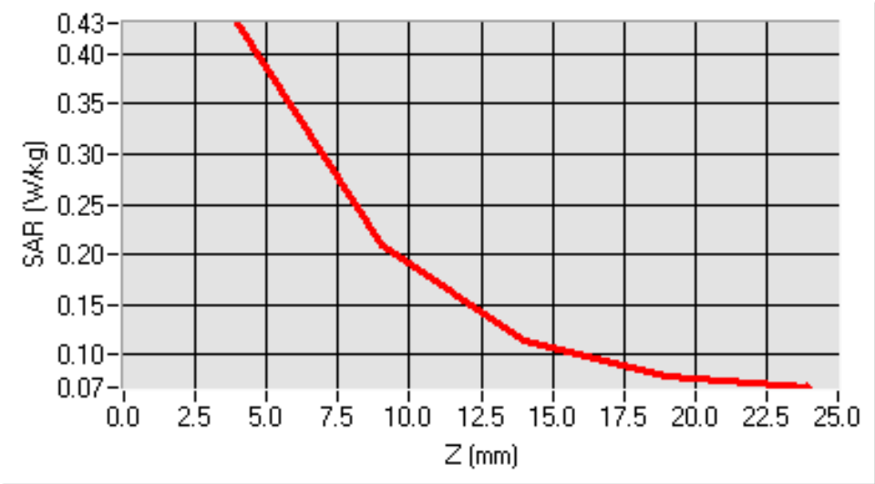
SAR, Z Axis Scan (X = 9, Y = 0)
