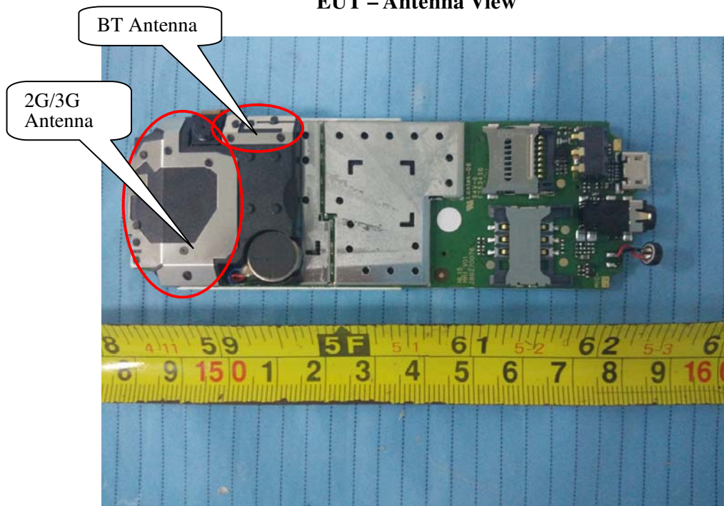
EUT – Antenna View
