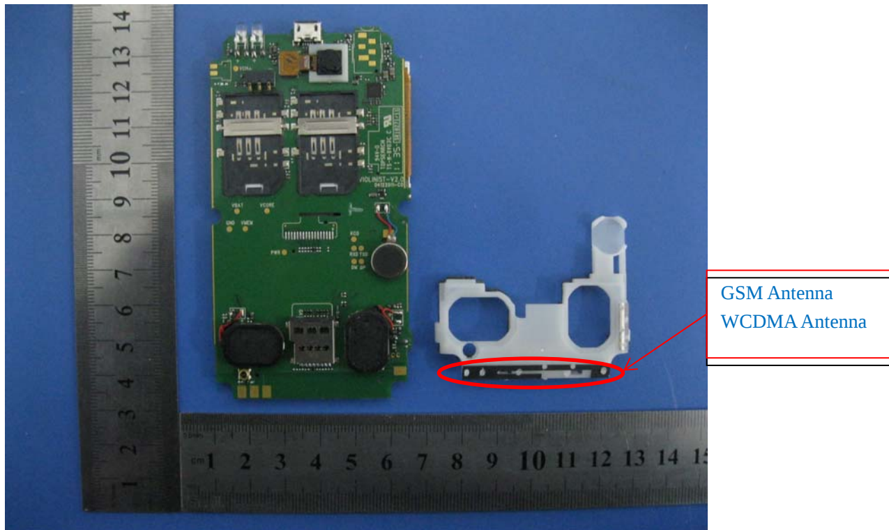
GSM Antenna, WCDMA Antenna - Top View
