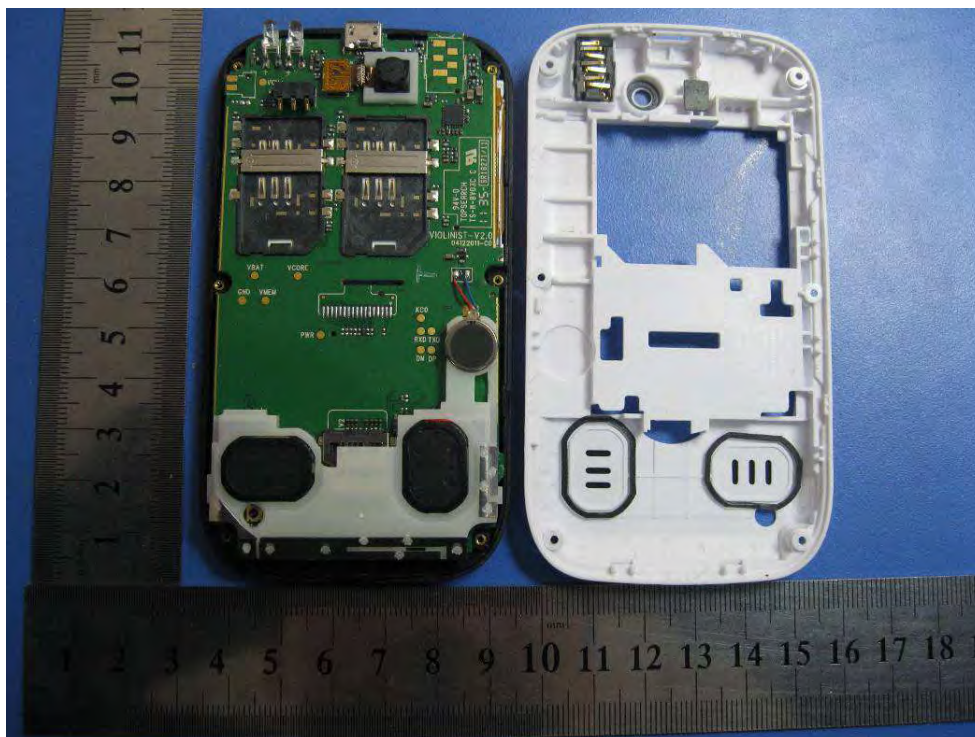
EUT – Main Board with Antenna Top View
