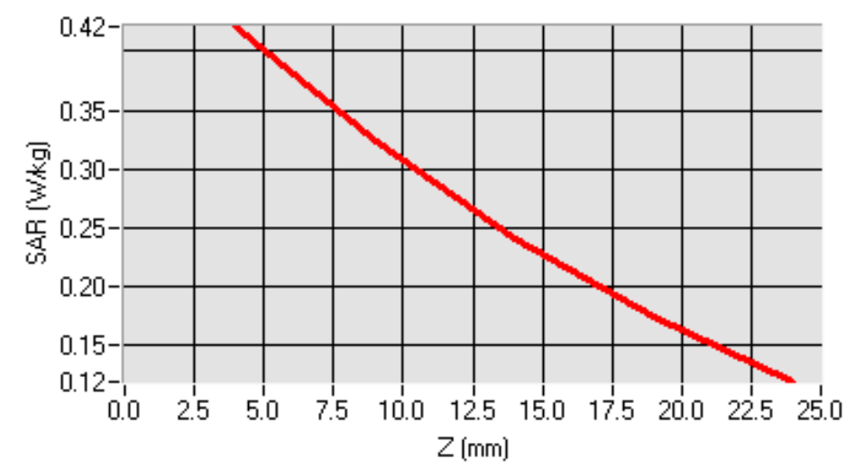
SAR, Z Axis Scan (X = -13, Y = 0)
