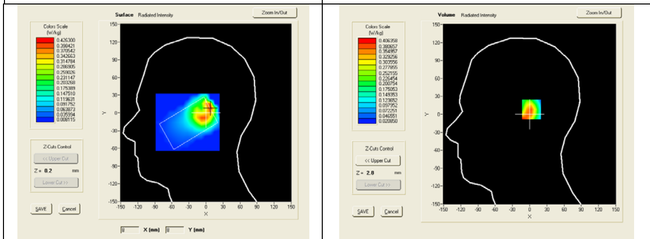
SAR, Z Axis Scan (X = 8, Y = 8)
