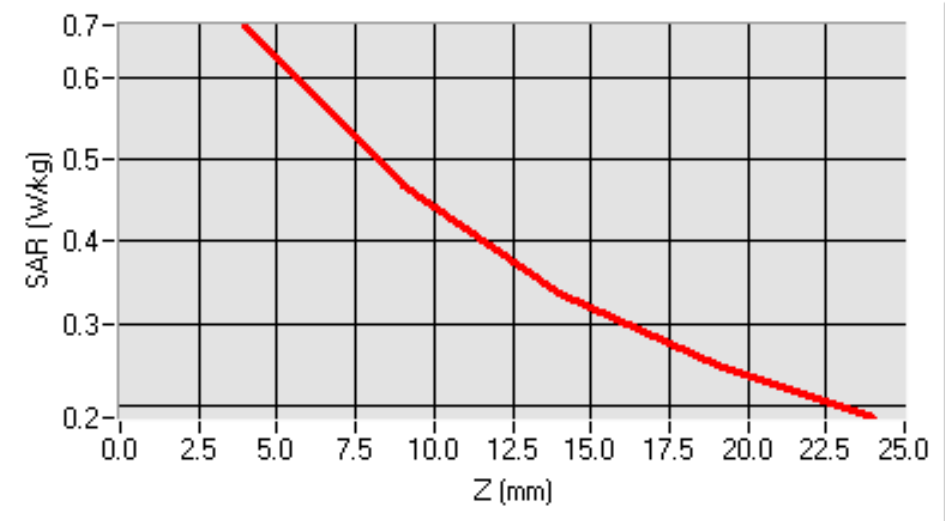
SAR, Z Axis Scan (X = -17, Y = -1)
