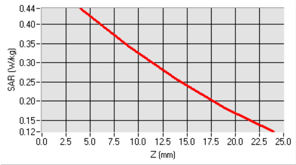
SAR, Z Axis Scan (X = -8, Y = -1)
