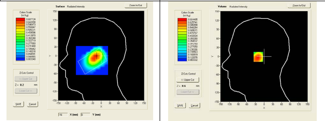
SAR, Z Axis Scan (X = -17, Y = -1)
