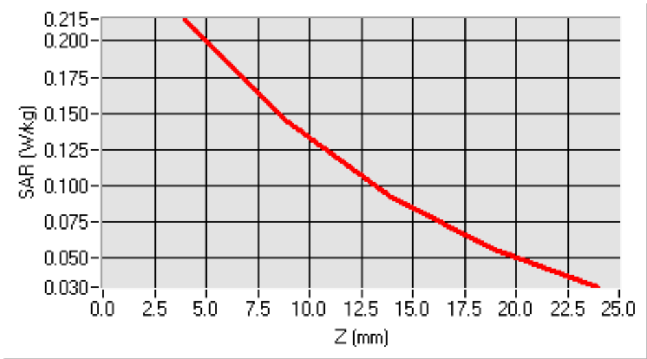
SAR, Z Axis Scan (X = 11, Y = -40)
