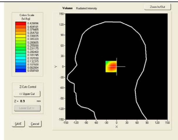
SAR, Z Axis Scan (X = -13, Y = 0)
