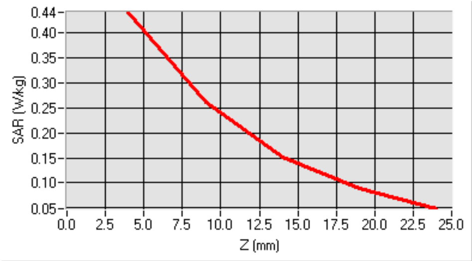
SAR, Z Axis Scan (X = -10, Y = 6)
