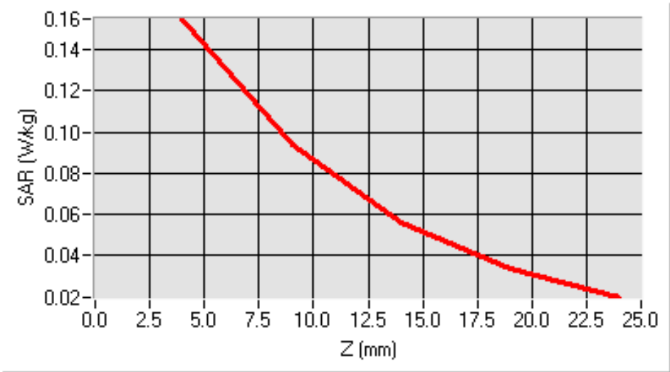
SAR, Z Axis Scan (X = 16, Y = -22)
