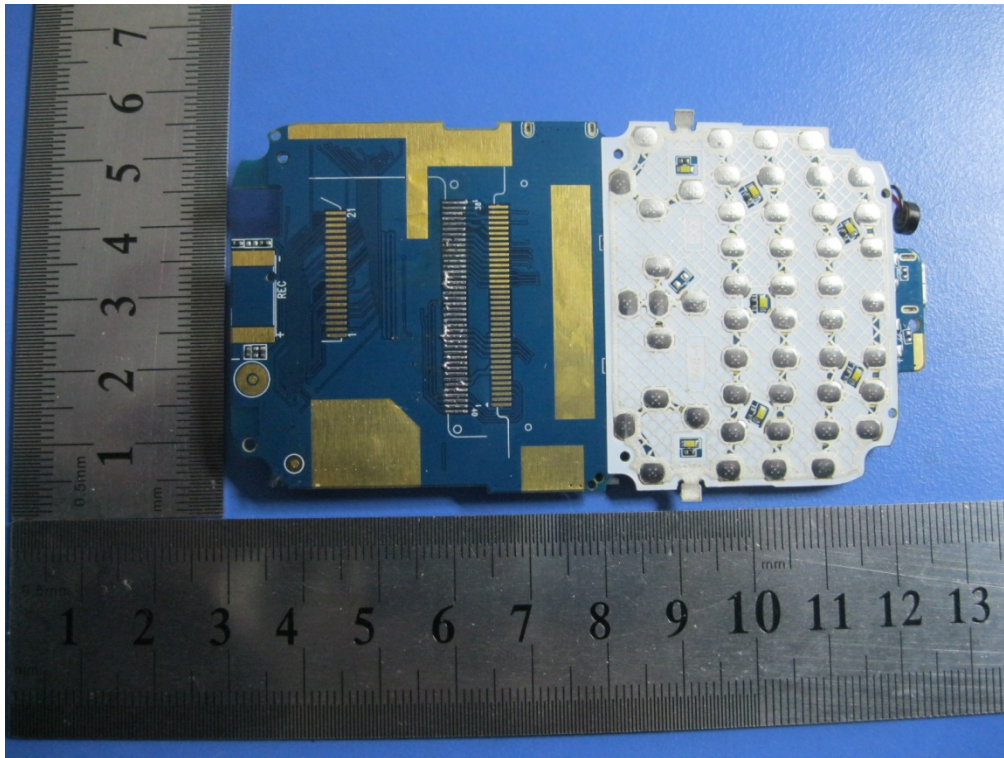
Front View of Main PCB
