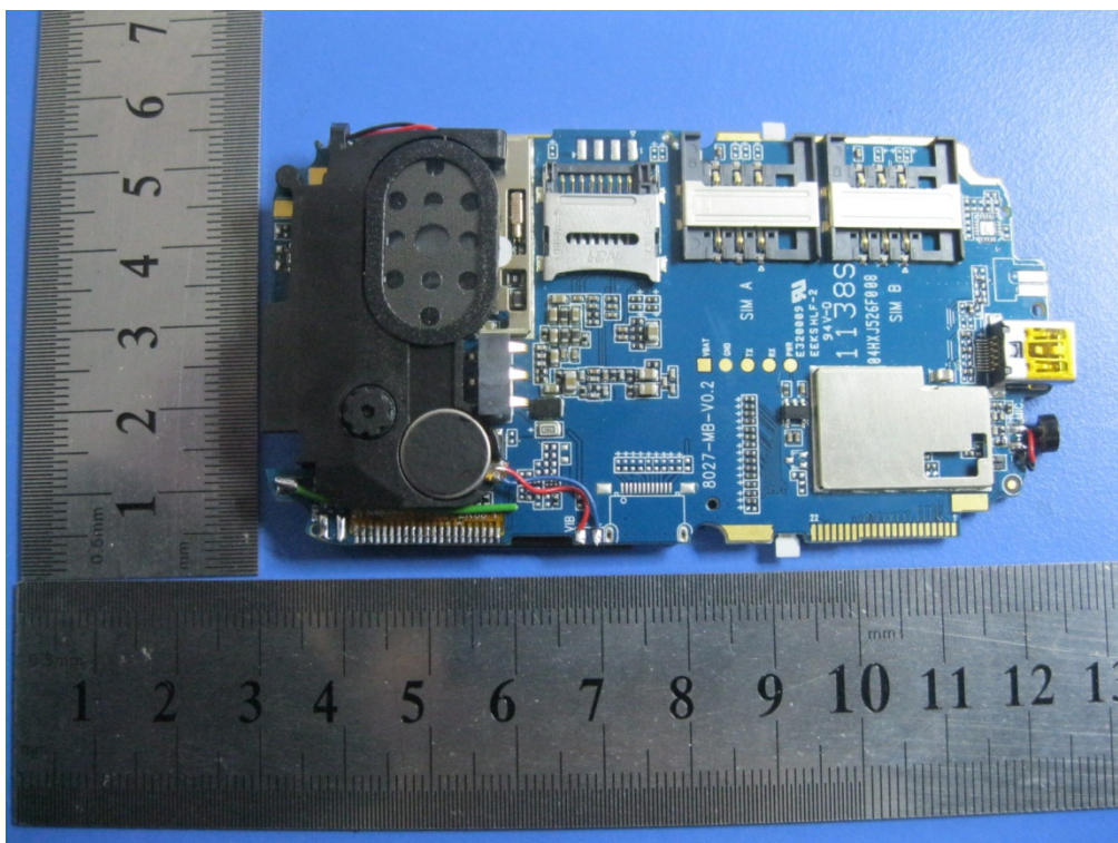
Rear View of EUT Internal
