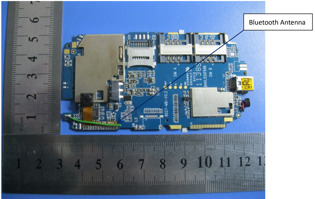
Front View of Bluetooth Antenna
