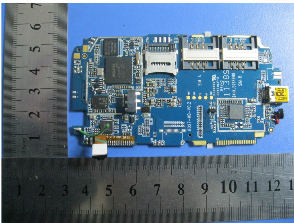
Rear View of PCB Shielding off
