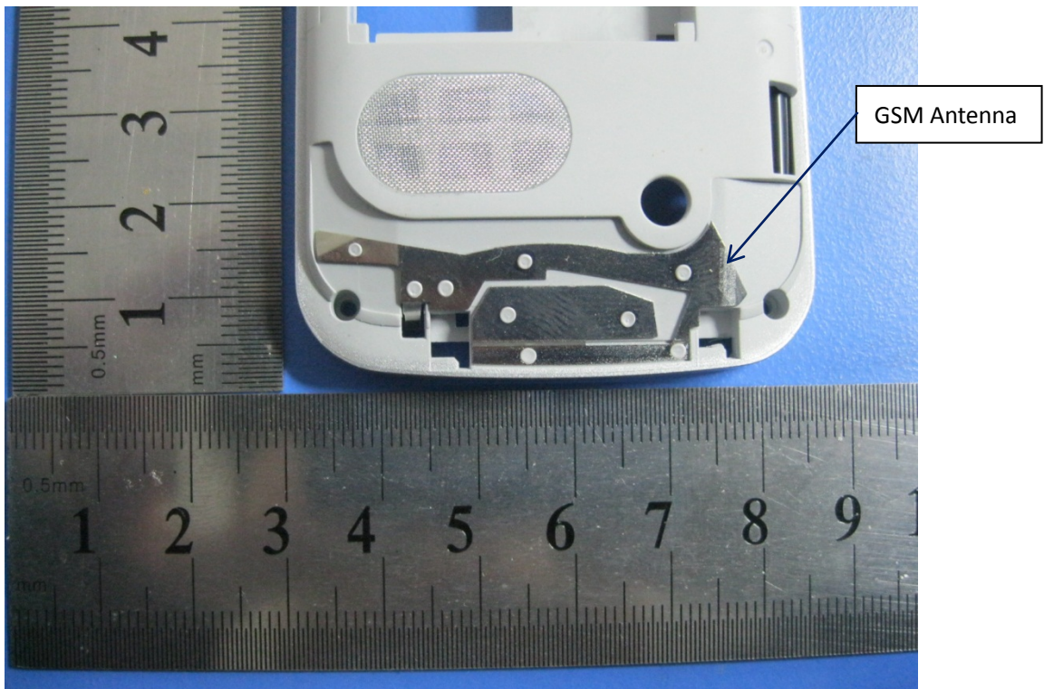
Front View of GSM Antenna
