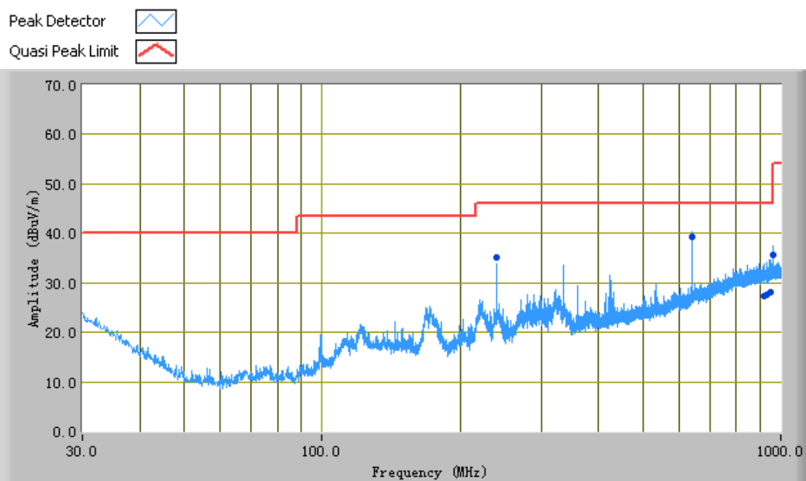
Horizontal Polarity Plot at 120Vac, 60Hz
