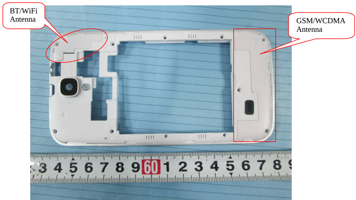
EUT – Antenna View
