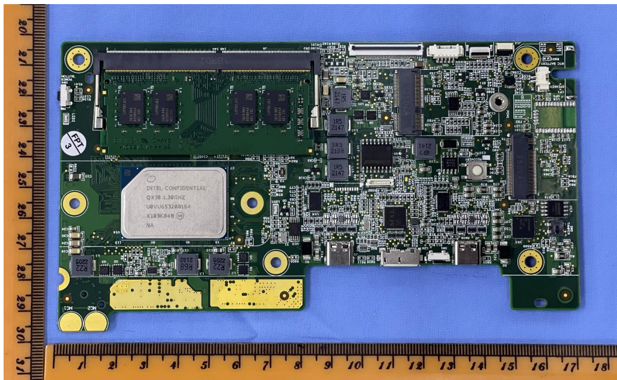
(Mainboard Front View)
