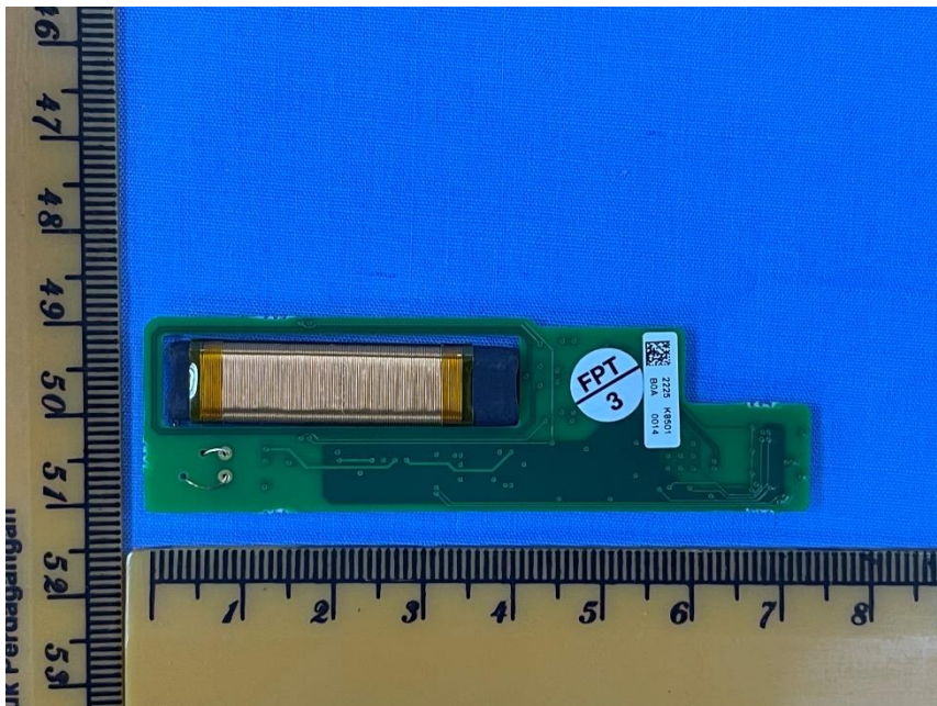
(RFID Reader PCBA)
