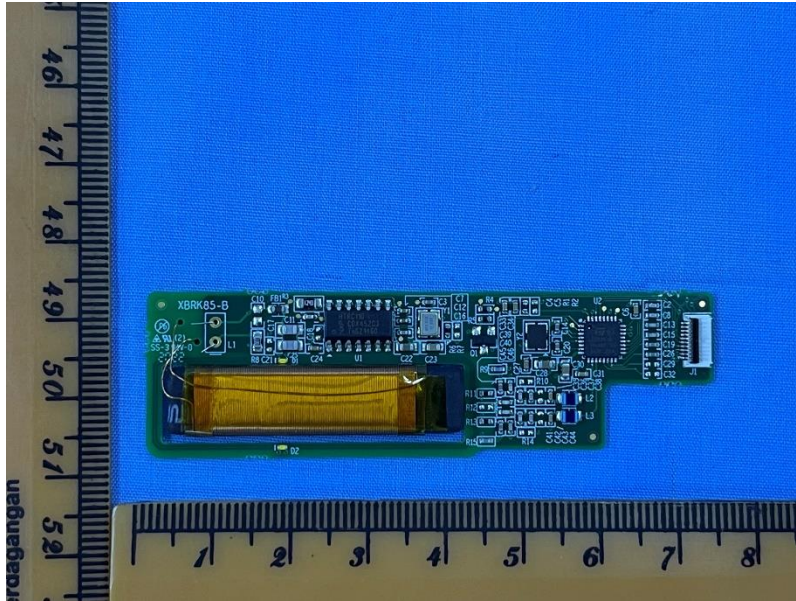
(RFID PCBA Trace)
