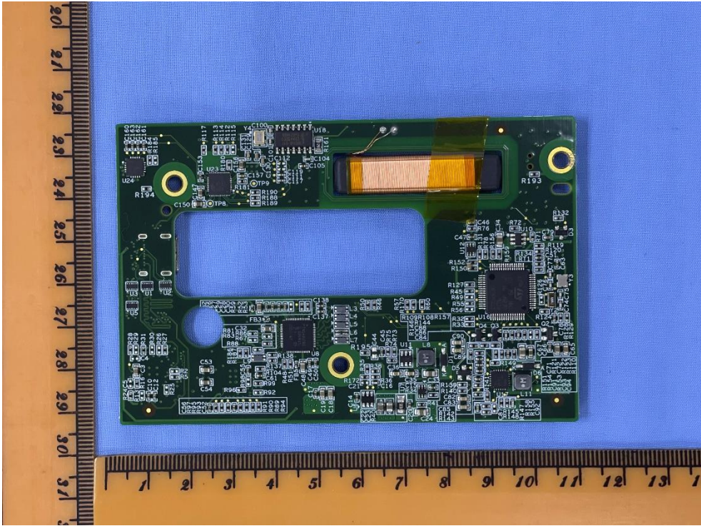
front view for PCBA
