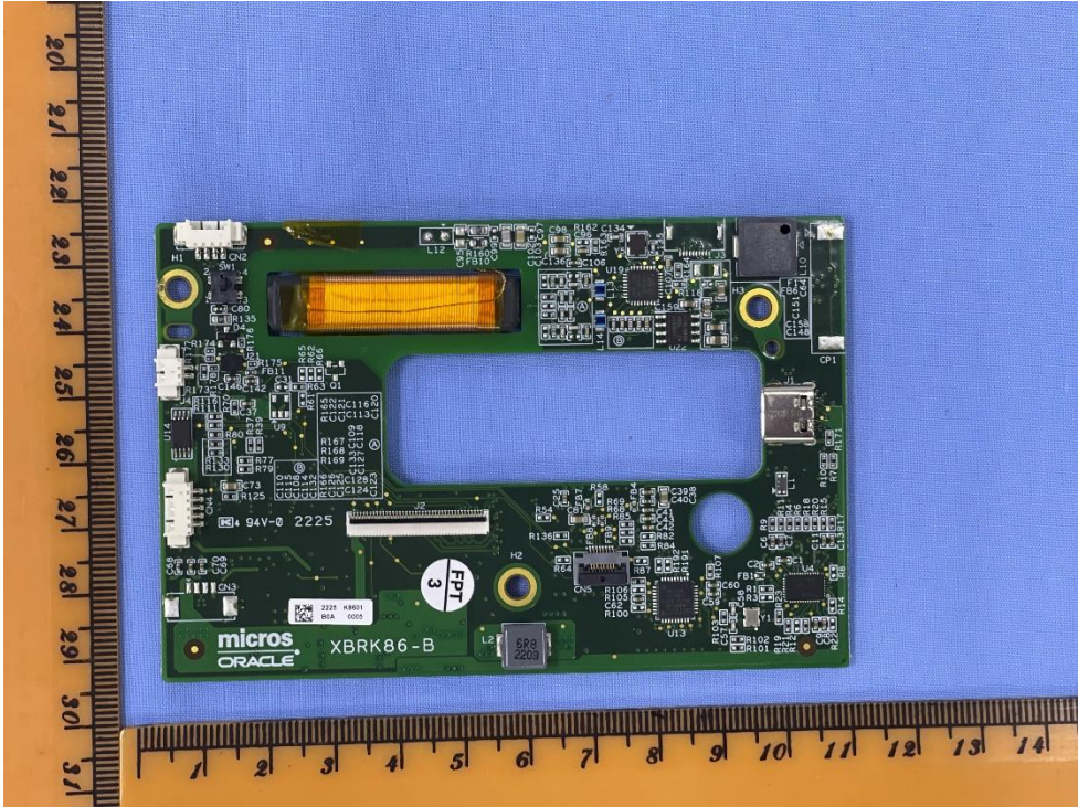
back view for PCBA
