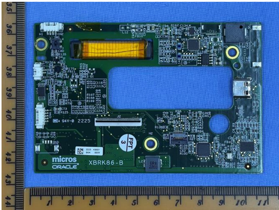
(Mainboard PCBA)
