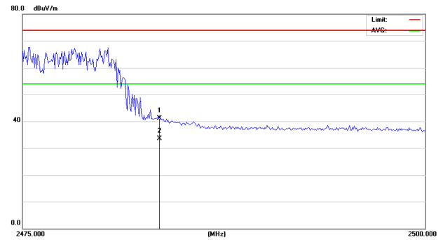
8-DPSK: Band Edge-High Channel -H
