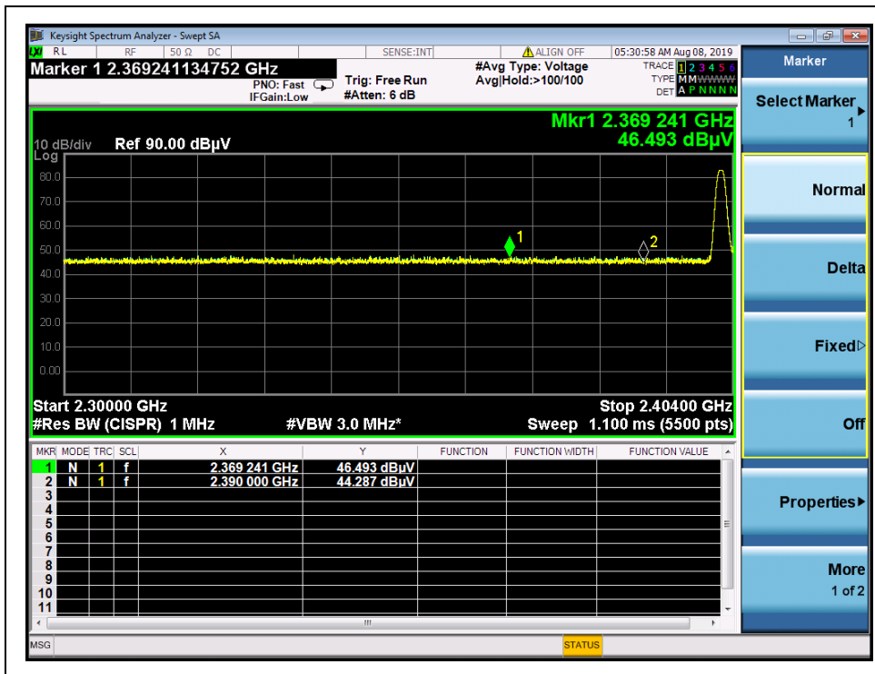
(Channel = 0, AVERAGE, GFSK)
