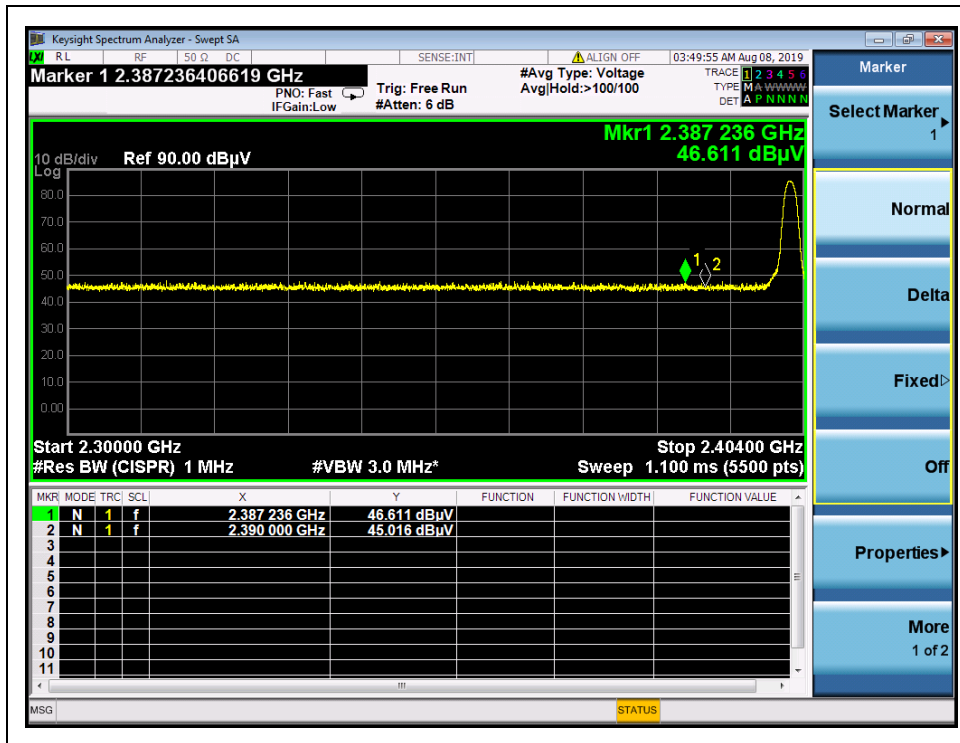
(Channel = 0, AVERAGE, \pi/4 -DQPSK)
