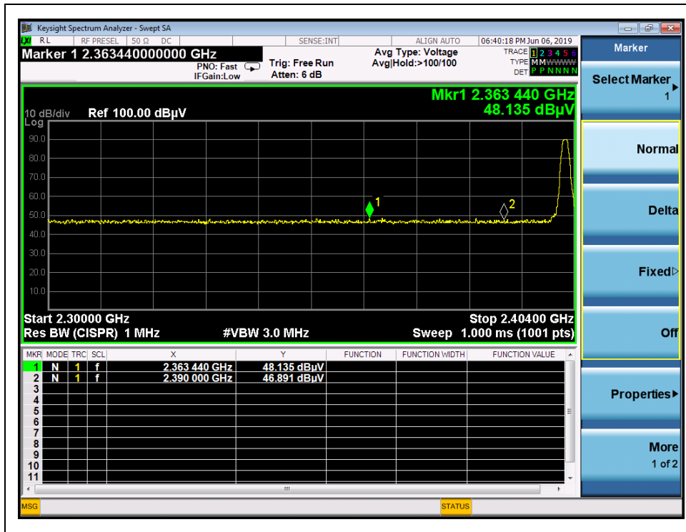
(Channel = 0, PEAK, GFSK)
