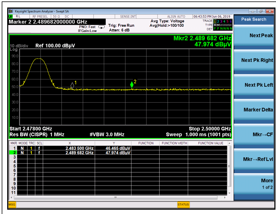
(Channel = 78, PEAK, GFSK)
