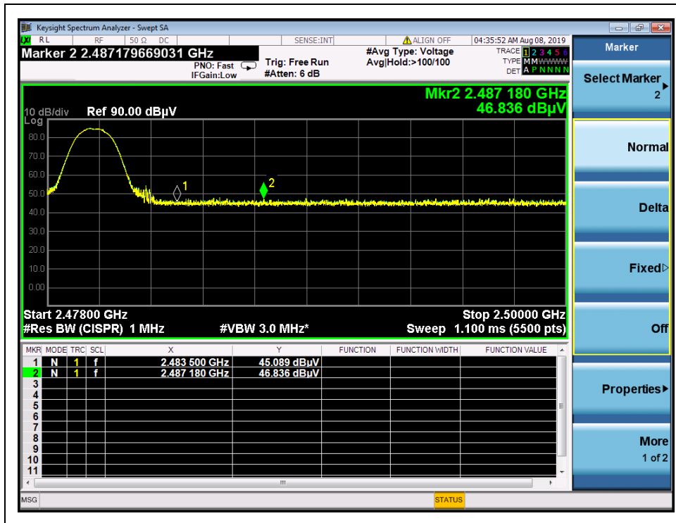
(Channel = 78, AVERAGE, \pi/4 -DQPSK)
