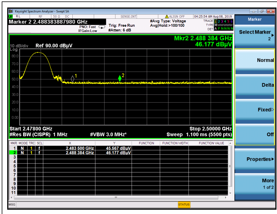
(Channel = 78, AVERAGE, 8-DPSK)
