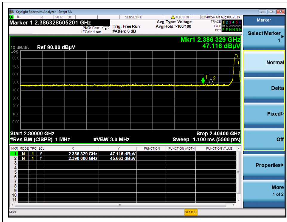
(Channel = 0, PEAK, \pi/4 -DQPSK)
