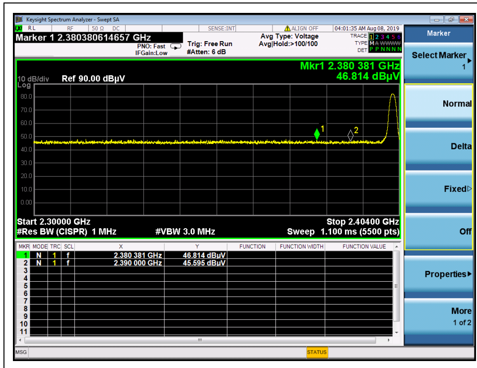
(Channel = 0, PEAK, 8-DPSK)
