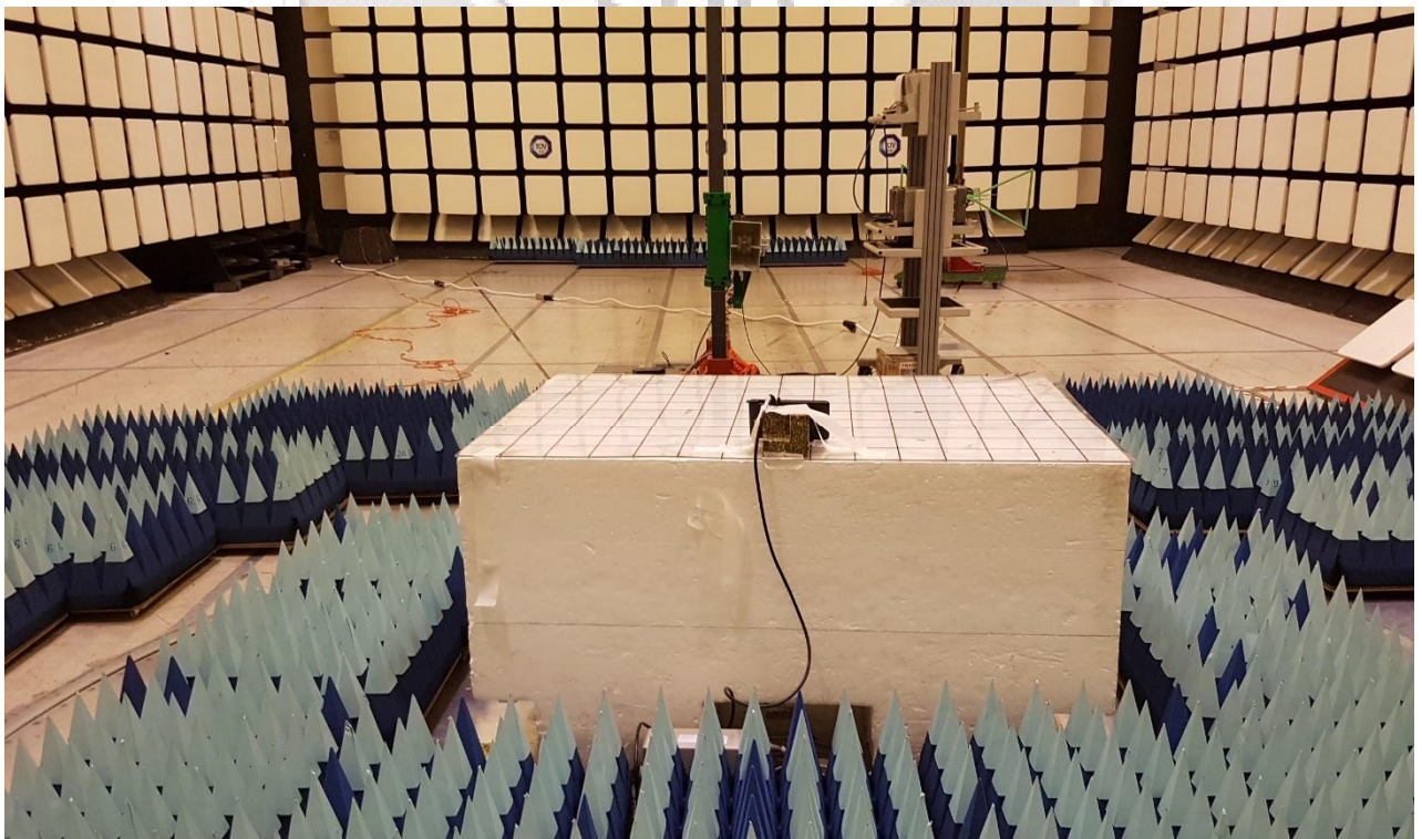
Receiver Spurious Emissions Test Setup (Rear View)
