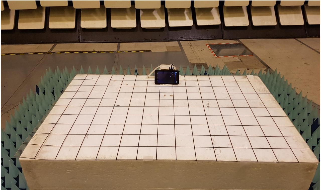
Receiver Spurious Emissions Test Setup (Front View)
