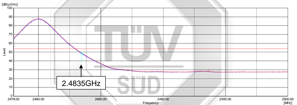
Plot 6 – Average Plot at Upper Band Edge at 2.4835GHz
