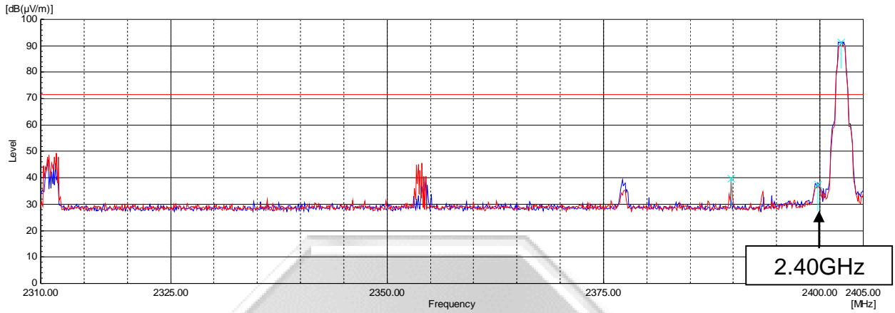
Plot 1 – Lower Band Edge at 2.4000GHz
