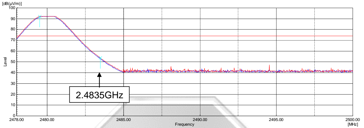
Plot 5 – Peak Plot at Upper Band Edge at 2.4835GHz
