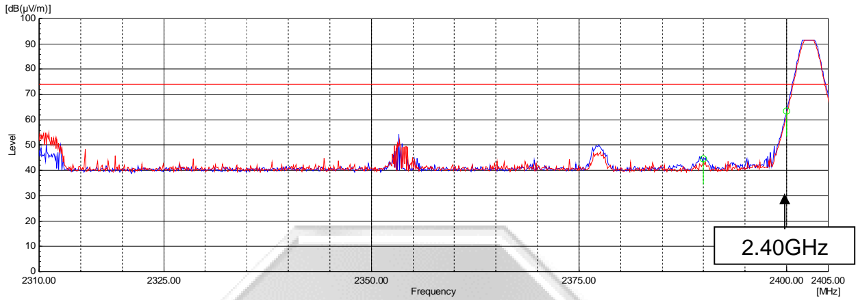
Plot 3 – Peak Plot at Lower Band Edge at 2.4000GHz
