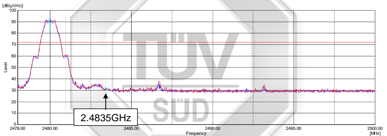
Plot 2 – Upper Band Edge at 2.4835GHz
