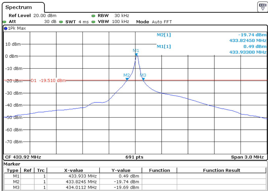
Channel 01: 433.92MHz
