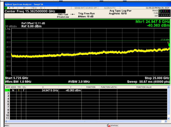
Spurious Emission:5725~25000.0 MHz IEEE 802.11ac Channel 100 20MHz Antenna 0
