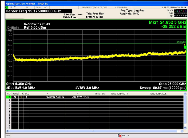
Spurious Emission:5350~25000.0 MHz IEEE 802.11ac Channel 52 20MHz Antenna 0
