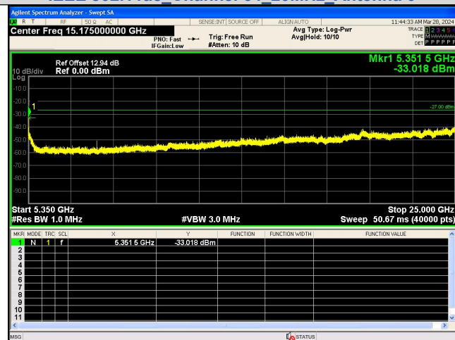
Spurious Emission:5350~25000.0 MHz IEEE 802.11ac Channel 64 20MHz Antenna 0
