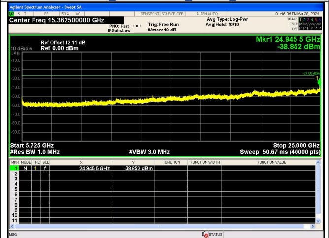
Spurious Emission:5725~25000.0 MHz IEEE 802.11n Channel 100 20MHz Antenna 0
