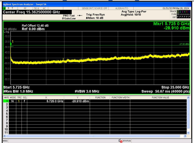
Spurious Emission:5725~25000.0 MHz IEEE 802.11n Channel 140 20MHz Antenna 0
