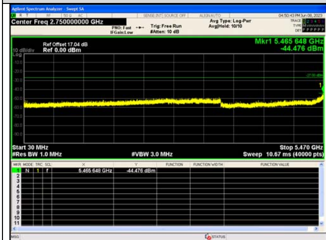
Spurious Emission:30.0~5470 MHz IEEE 802.11ac_Channel 100_20MHz_Antenna 0
