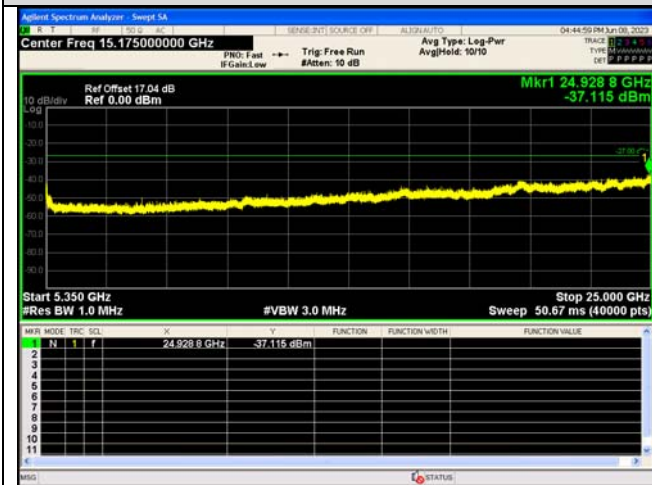
Spurious Emission:5350~25000.0 MHz IEEE 802.11ac_Channel 58_80MHz_Antenna 0
