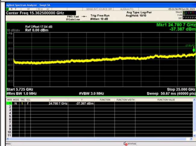
Spurious Emission:5725~25000.0 MHz IEEE 802.11n_Channel 134_40MHz_Antenna 0
