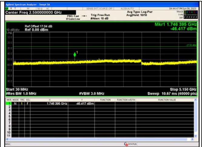
Spurious Emission:30.0~5150 MHz IEEE 802.11ac_Channel 58_80MHz_Antenna 0
