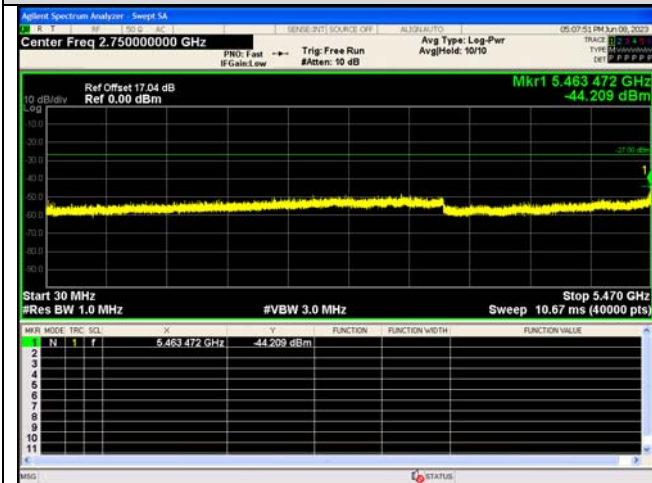
Spurious Emission:30.0~5470 MHz IEEE 802.11ac_Channel 122_80MHz_Antenna 0
