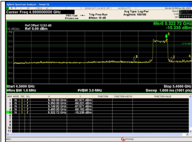
Out Of Band Emission IEEE 802.11ac_Channel 58_80MHz_Antenna 0
