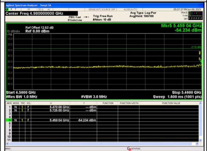
Out Of Band Emission IEEE 802.11ac_Channel 122_80MHz_Antenna 0
