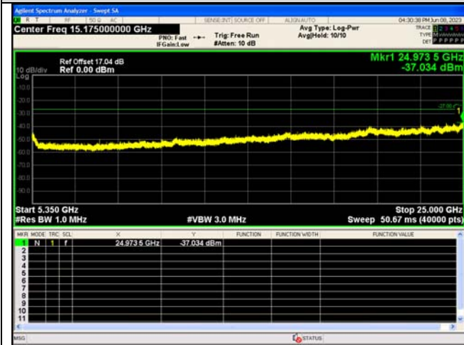
Spurious Emission:5350~25000.0 MHz IEEE 802.11ac_Channel 52_20MHz_Antenna 0
