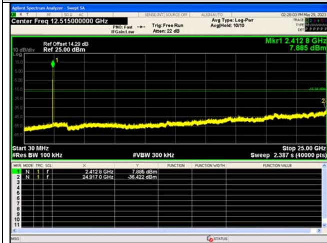
Spurious Emission
