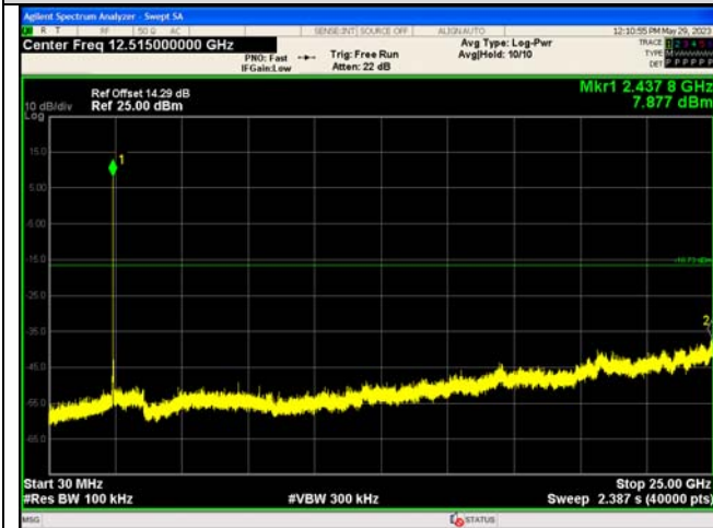
Spurious Emission
