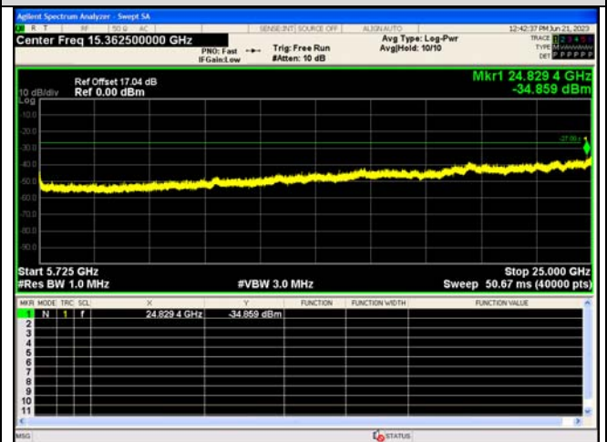
Spurious Emission:5725~25000.0 MHz IEEE 802.11ac_Channel 122_80MHz_Antenna 0
