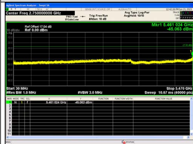
Spurious Emission:30.0~5470 MHz IEEE 802.11ac_Channel 122_80MHz_Antenna 0
