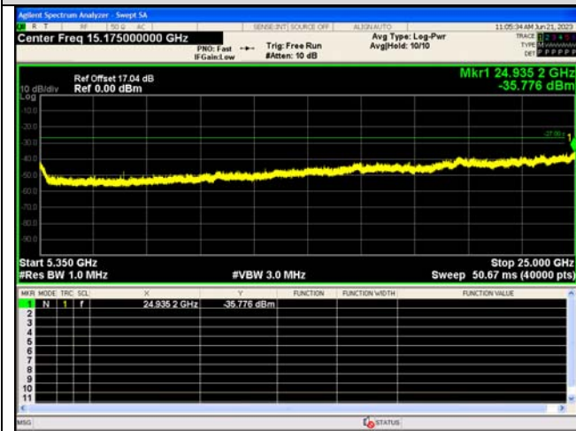
Spurious Emission:5350~25000.0 MHz IEEE 802.11n_Channel 52_20MHz_Antenna 0
