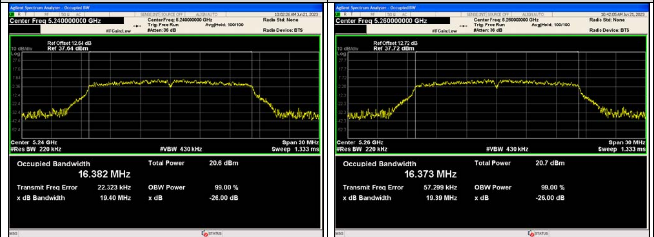
IEEE 802.11a_Channel 48_20MHz_Antenna 0
