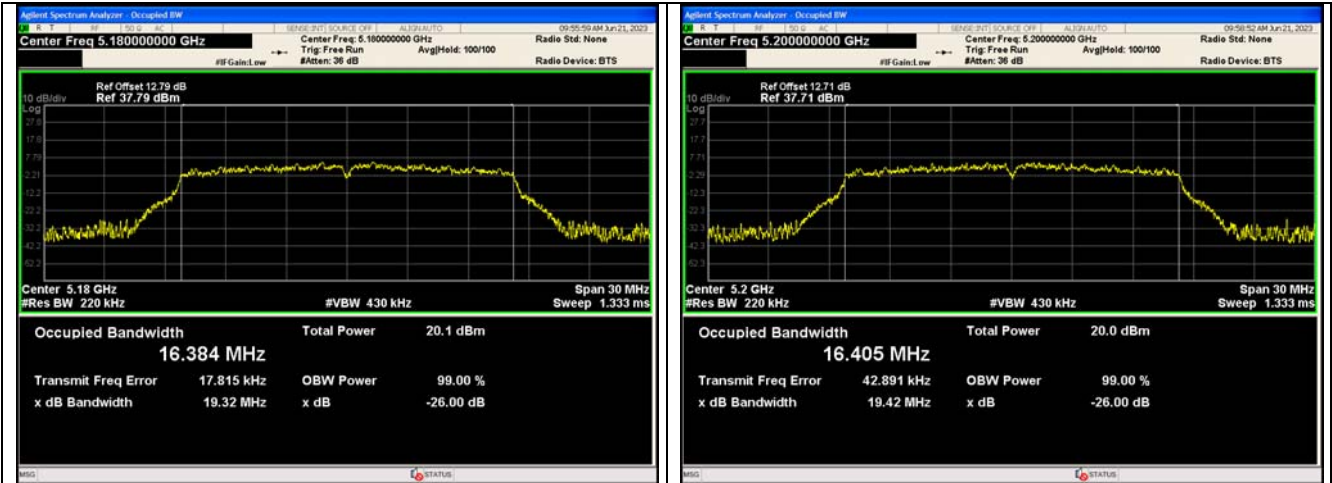
IEEE 802.11a_Channel 36_20MHz_Antenna 0
