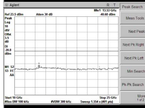
802.11g Mode, Ch1
