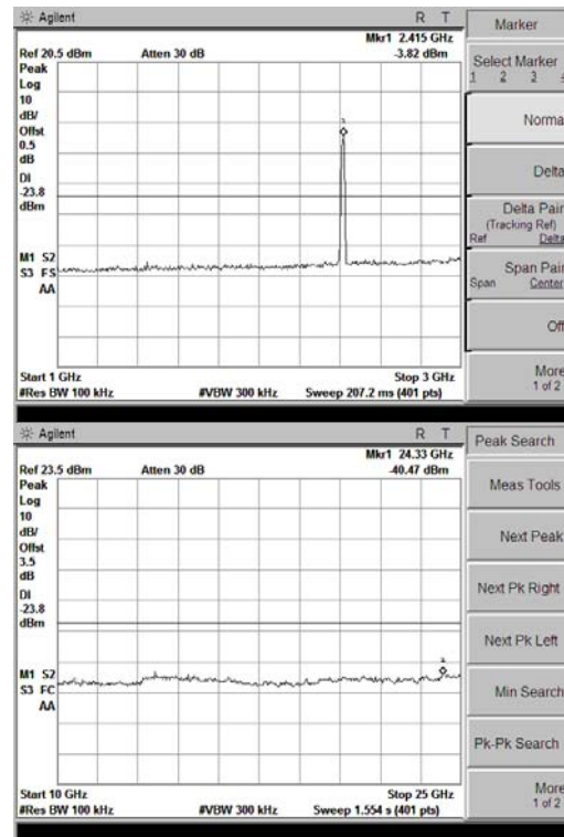
802.11 n(20M) Mode, Ch1
