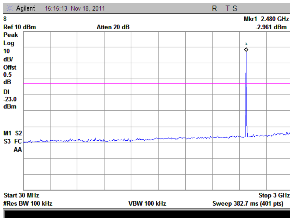
(Plot F.1: Channel = 78, 30MHz to 3GHz @ \pi/4 -DQPSK)
