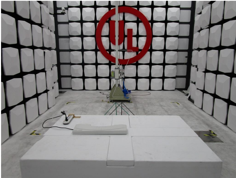
30-1000MHz Front
