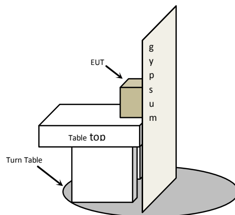
SETUP diagram
