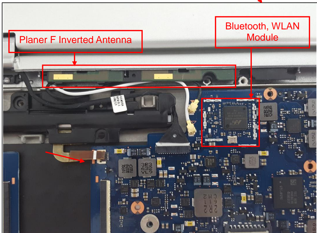
The transmit antenna location and the WiFi component
