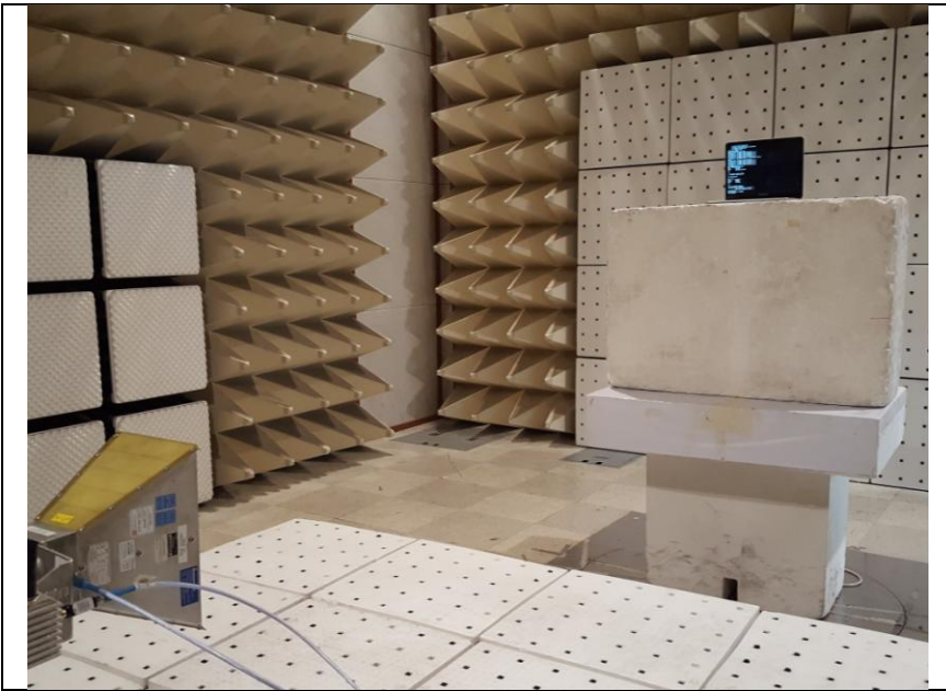
- Photo of Radiated Spurious Emission Test (Above 1 GHz)
