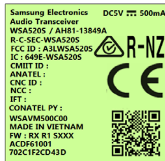
RX-Woofer
