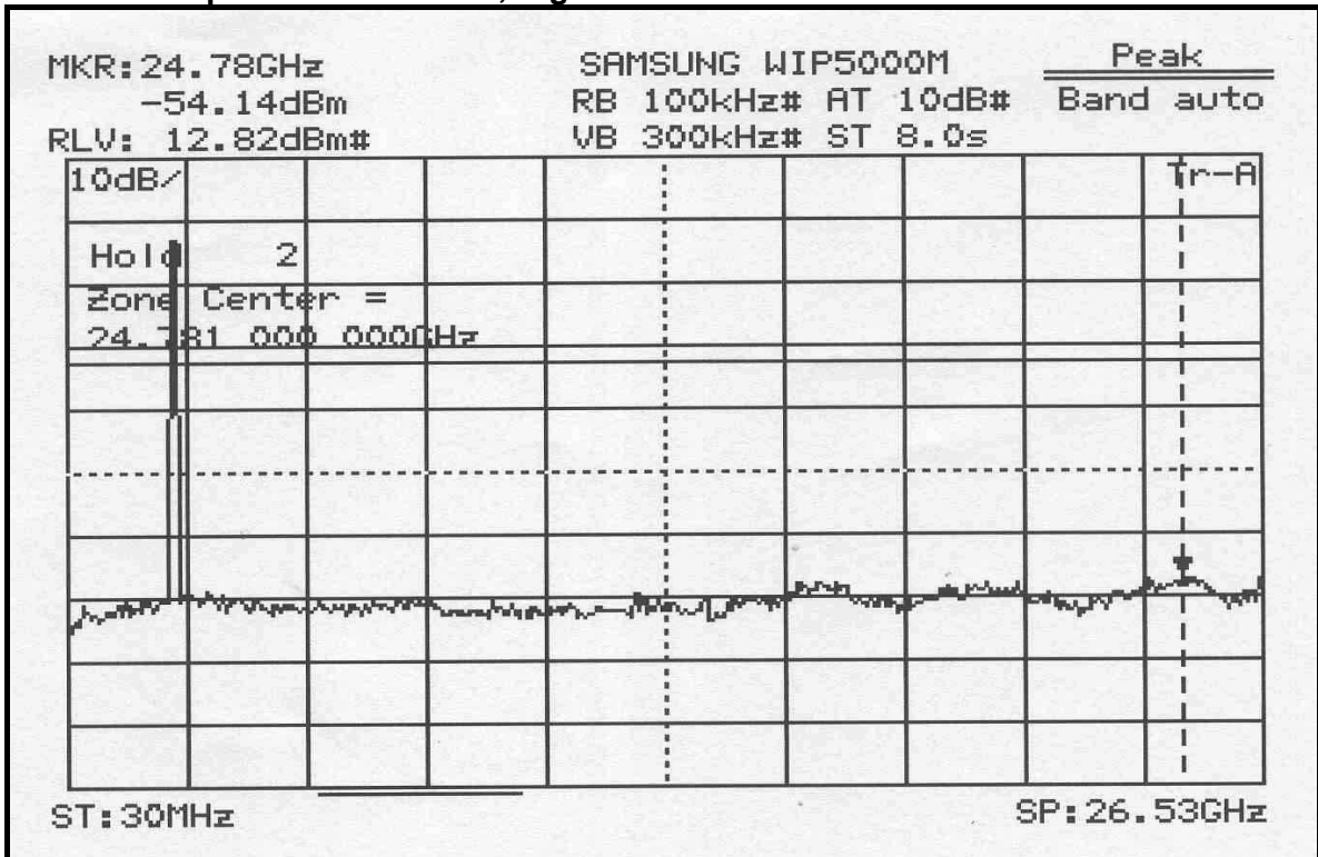
Conducted Spurious Emissions, High Channel
