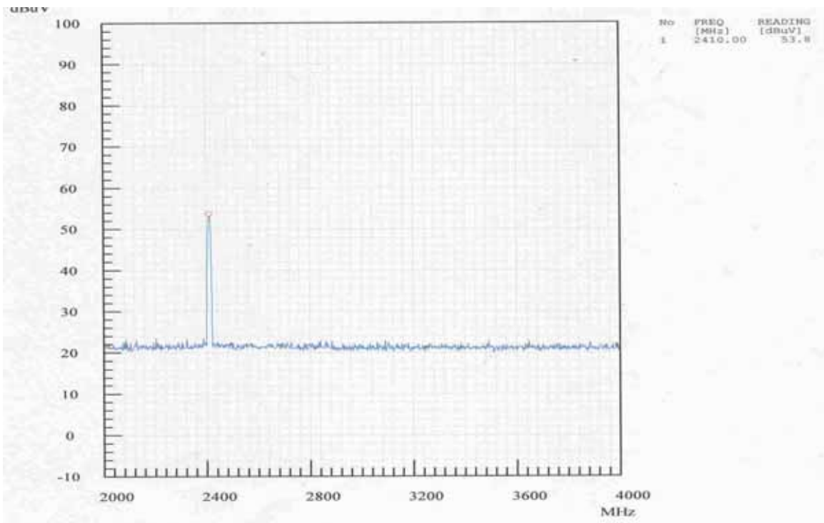
Radiated Spurious Emissions, low Channel(Vertical)
