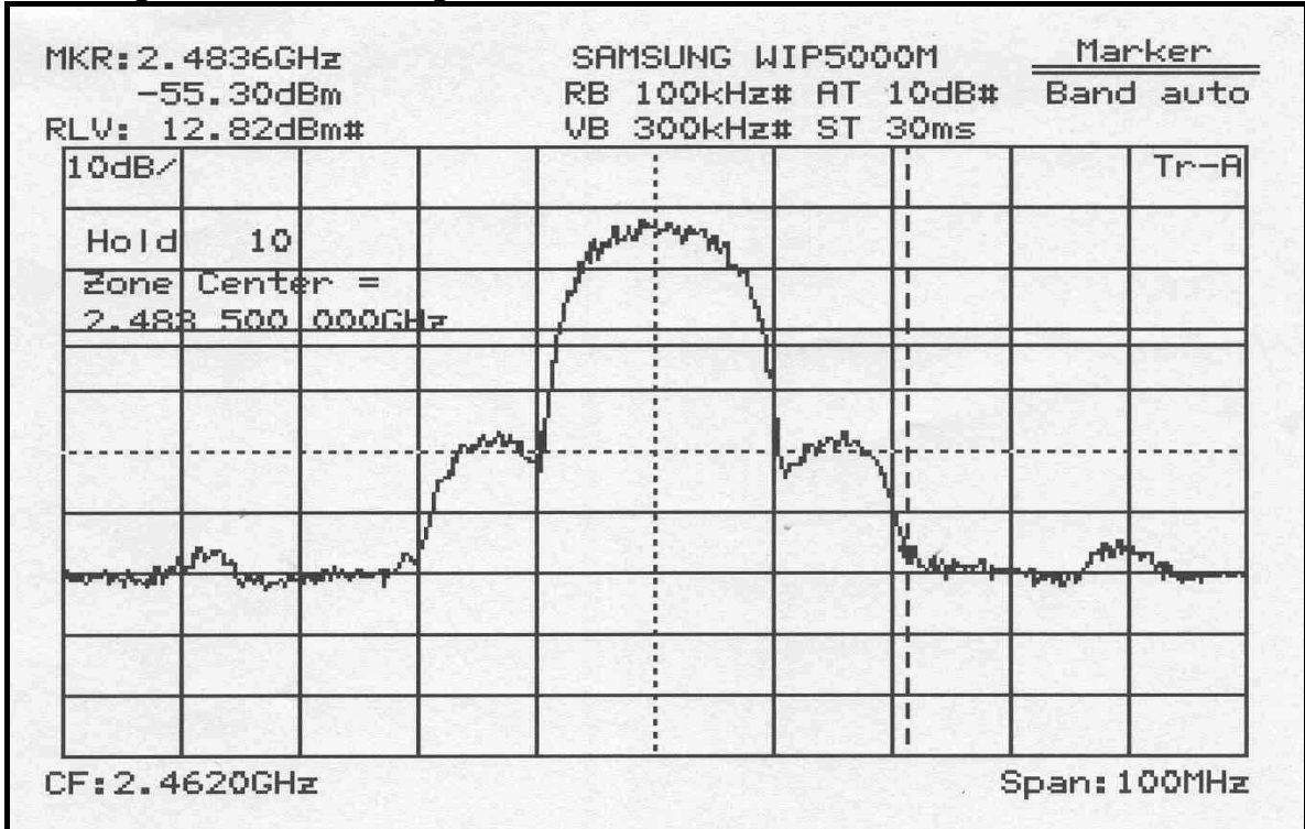
Band edge at 2.4835GHz, High Channel
