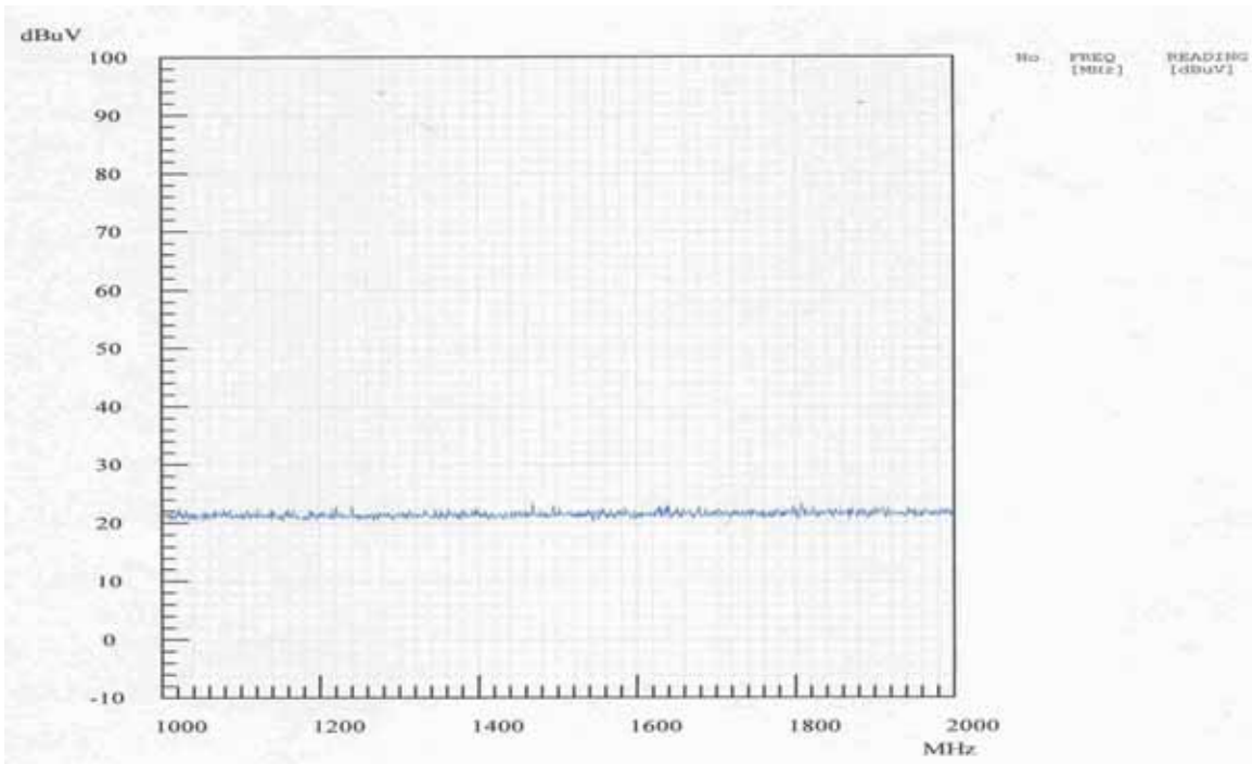
Radiated Spurious Emissions, low Channel(Vertical)
