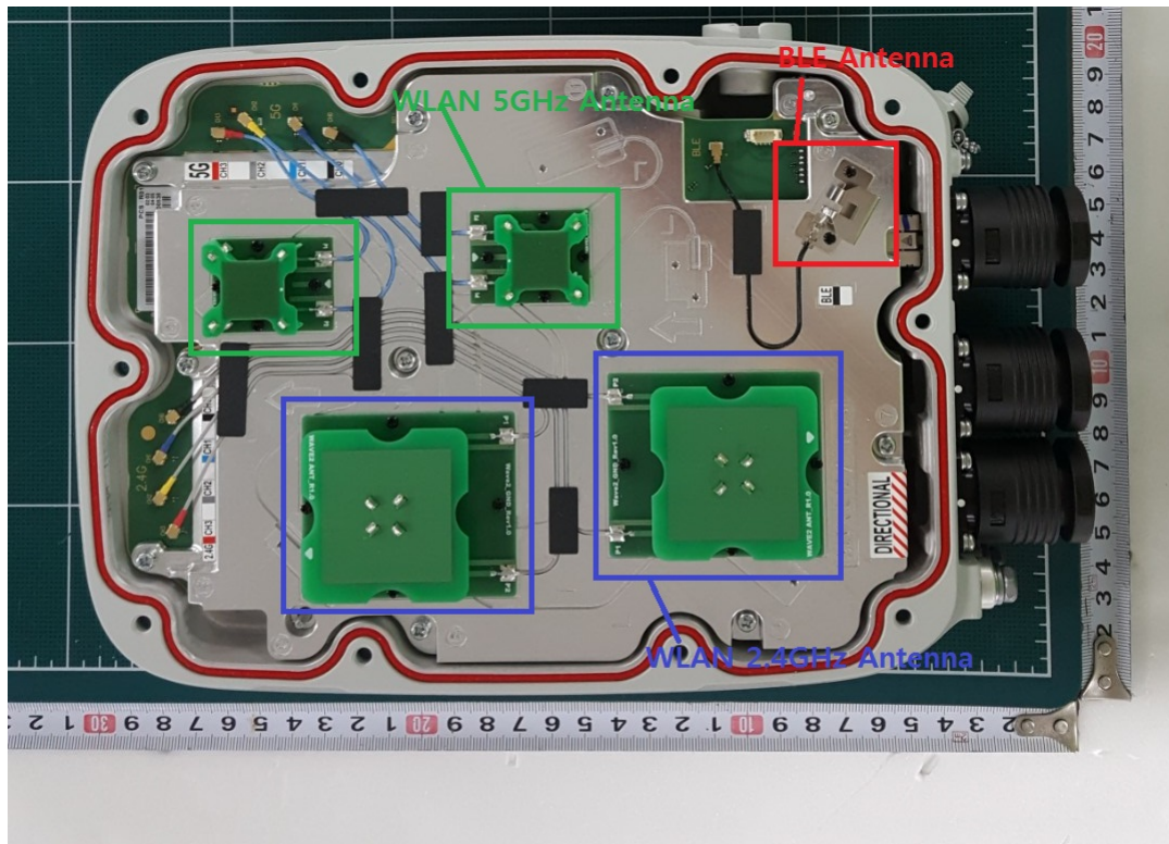
Antenna (WEA554d)
