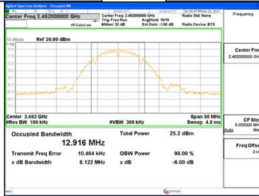
Ant 2_802.11b
