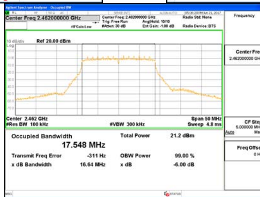
Ant 3_802.11n_HT20
