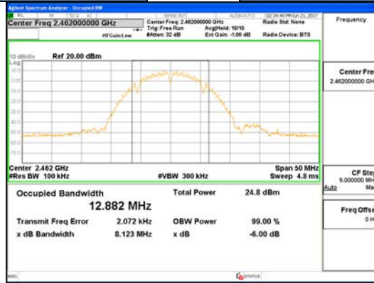
Ant 3_802.11b
