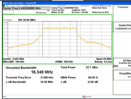
Ant 2_802.11g
