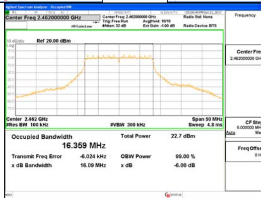
Ant 1_802.11g
