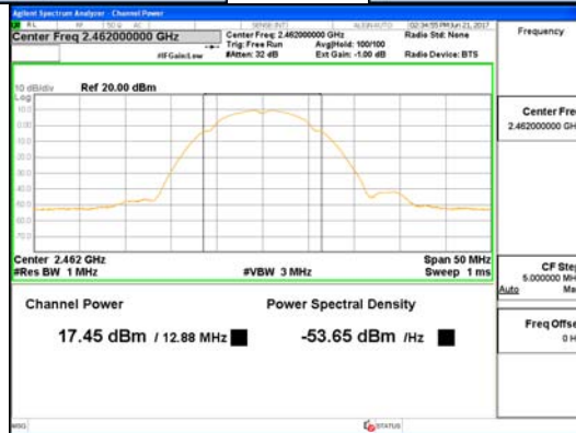
Ant 3_802.11b
