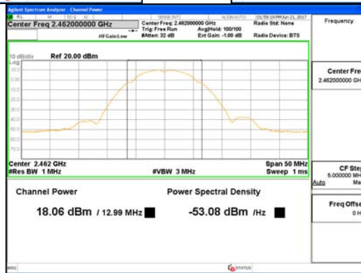
Ant 1_802.11b
