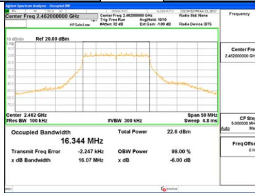
Ant 3_802.11g
