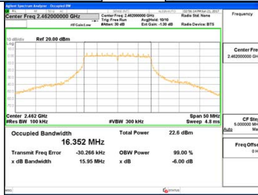
Ant 0_802.11g
