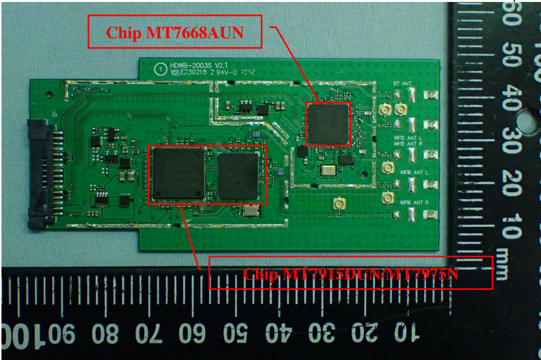
Figure 15 Internal View (Front View)
