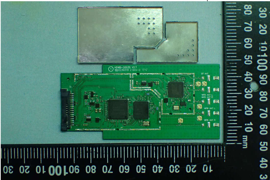
Figure 14 Internal View (Removed Shielded Case)
