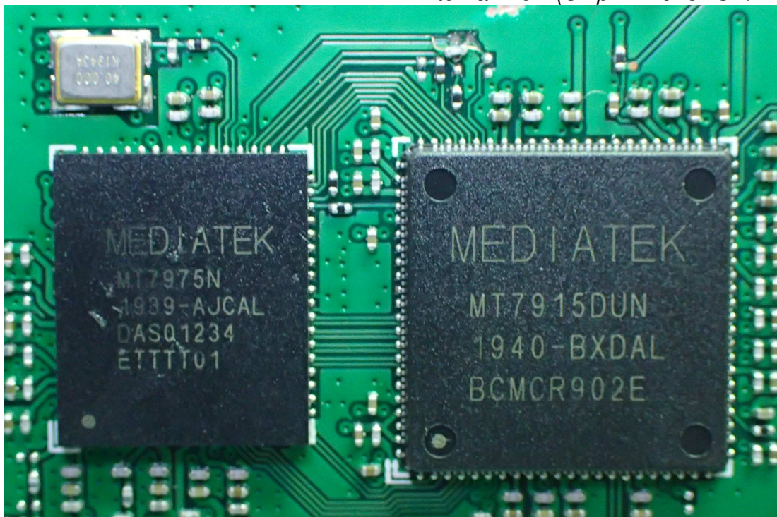
Figure 17 Internal View (Chip MT7915DUN/MT7975N)
