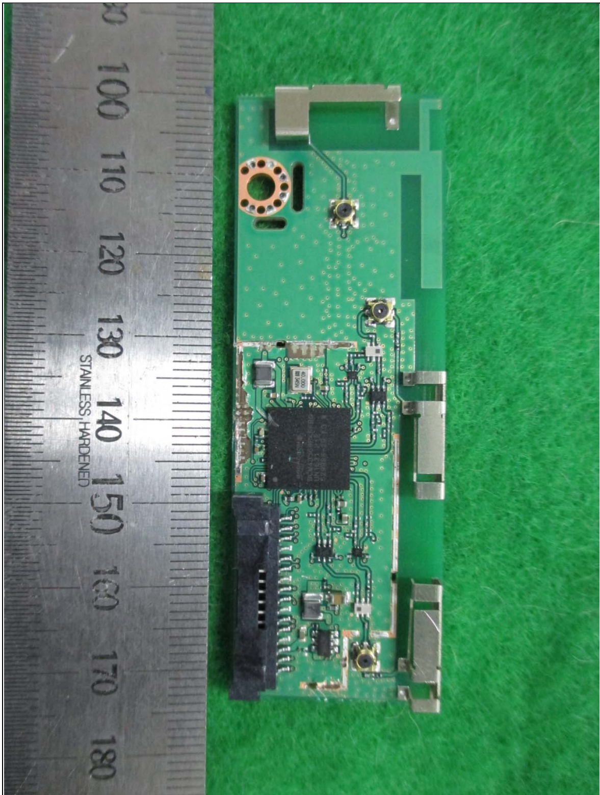
Front View of Main Board without shield can
