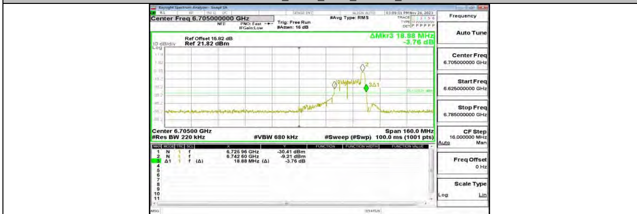
11AX80MIMO_ANT1_6705_26Tone_RU17
