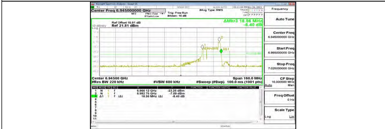
11AX80MIMO ANT1_6945_26Tone_RU36
