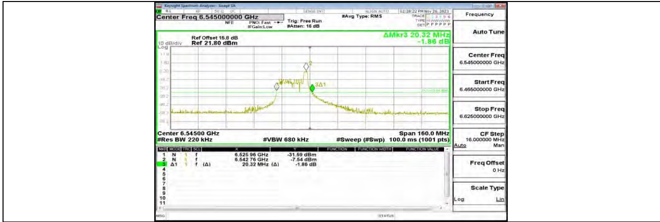
11AX80MIMO_ANT1_6545_26Tone_RU17
