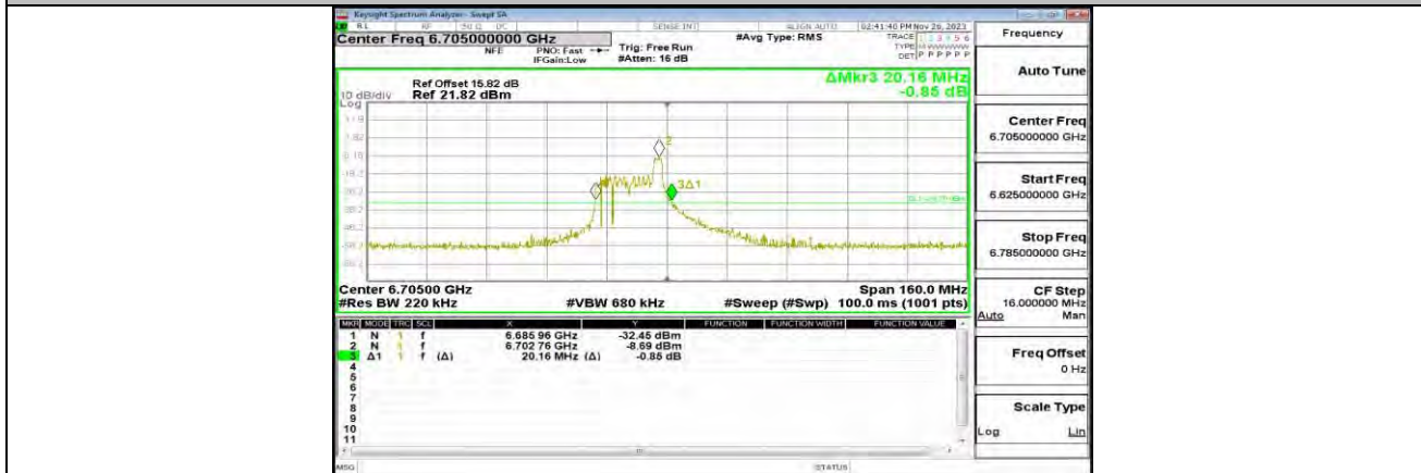
11AX80MIMO_ANT1_6705_26Tone_RU17
