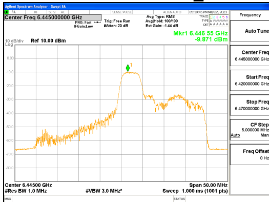
ANT L_802.11ax_HE40_52T_Mid_UNII 6
