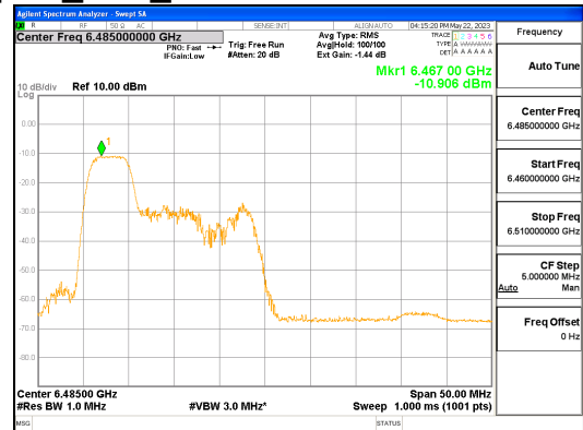
ANT R_802.11ax_HE40_52T_Low_UNII 6
