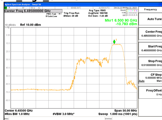
ANT R_802.11ax_HE40_52T_High_UNII 6
