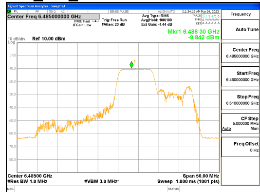
ANT L_802.11ax_HE40_106T_Mid_UNII 6
