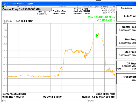
ANT R_802.11ax_HE40_52T_High_UNII 6
