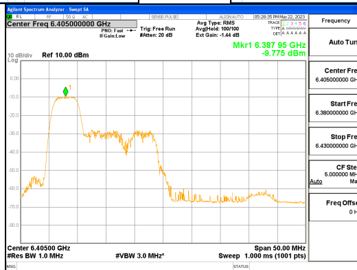
ANT L_802.11ax_HE40_52T_Low_UNII 5
