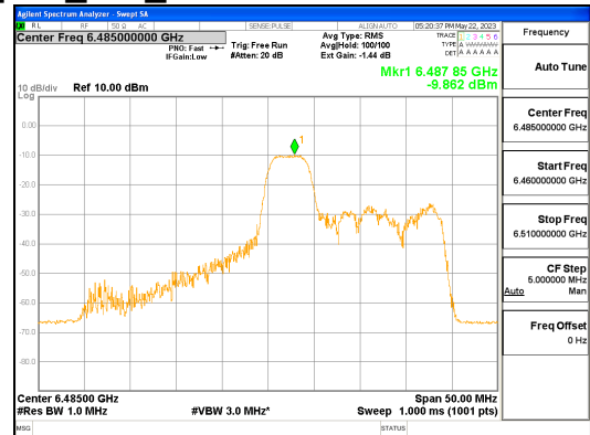
ANT L_802.11ax_HE40_52T_Mid_UNII 6
