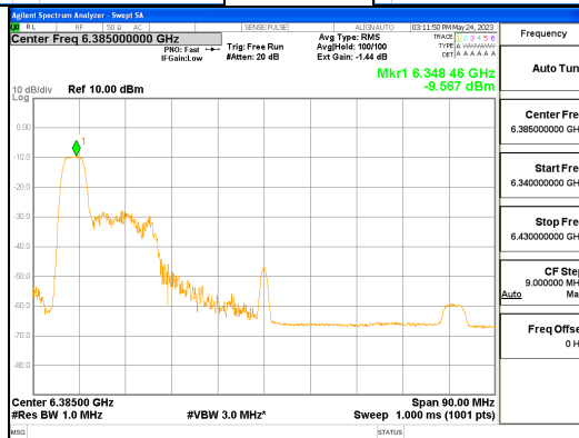
ANT L_802.11ax_HE80_52T_Low_UNII 5
