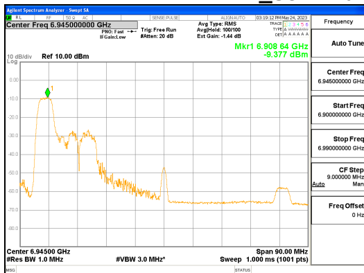
ANT L_802.11ax_HE80_52T_Low_UNII 8
