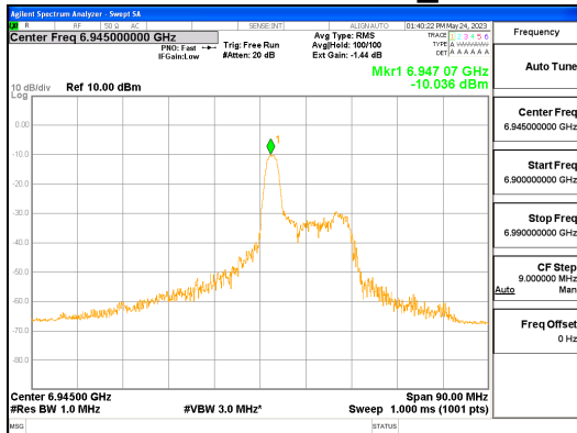
ANT R_802.11ax_HE80_26T_Mid_UNII 8
