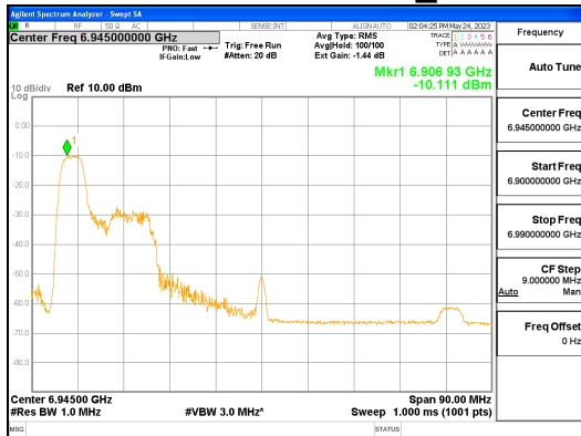
ANT R_802.11ax_HE80_52T_Low_UNII 8
