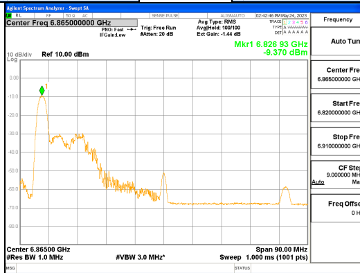
ANT L_802.11ax_HE80_26T_Low_UNII 7
