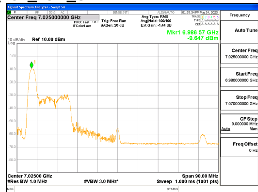
ANT R_802.11ax_HE80_26T_Low_UNII 8
