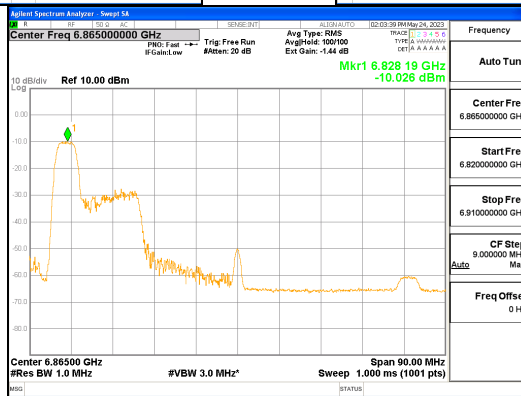
ANT R_802.11ax_HE80_52T_Low_UNII 7
