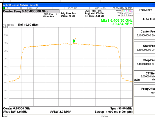
ANT R_802.11ax_HE40_484T_UNII 5
