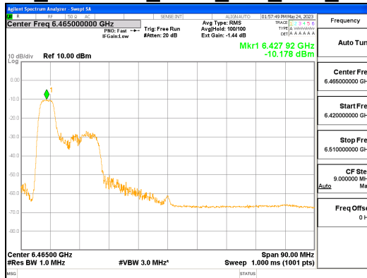
ANT R_802.11ax_HE80_52T_Low_UNII 6
