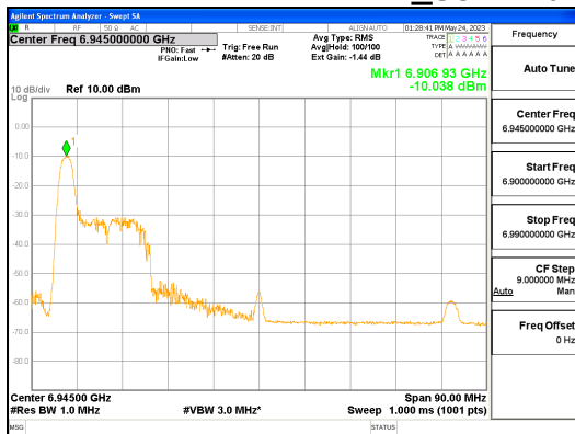
ANT R_802.11ax_HE80_26T_Low_UNII 8
