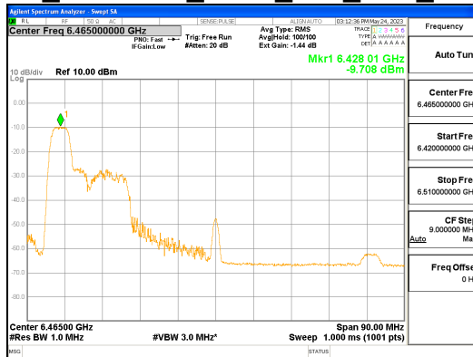
ANT L_802.11ax_HE80_52T_Low_UNII 6
