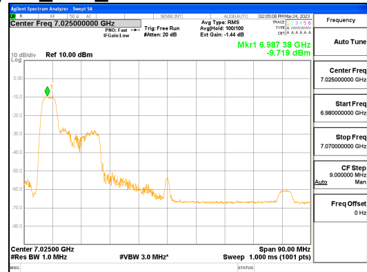
ANT R_802.11ax_HE80_52T_Low_UNII 8
