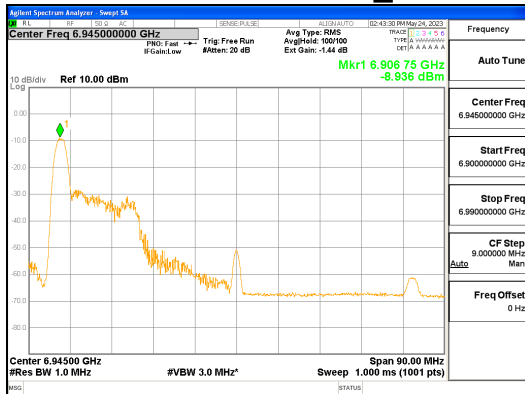
ANT L_802.11ax_HE80_26T_Low_UNII 8
