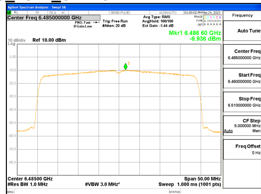
ANT L_802.11ax_HE40_484T_UNII 6
