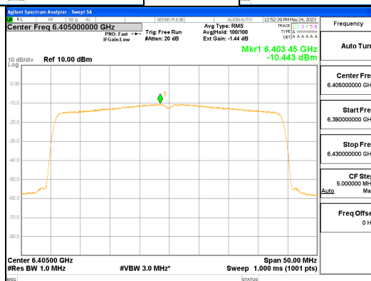
ANT L_802.11ax_HE40_484T_UNII 5
