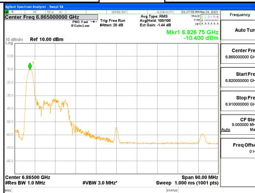
ANT R_802.11ax_HE80_26T_Low_UNII 7
