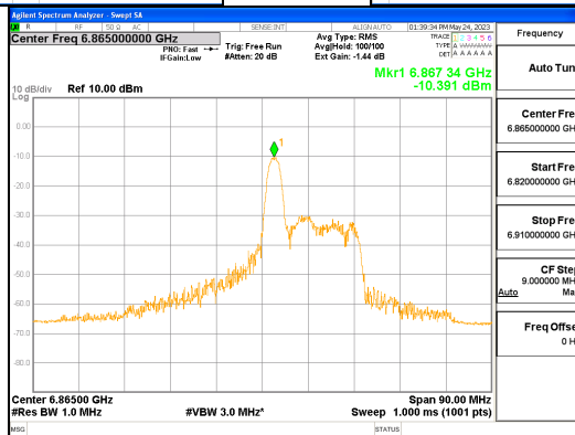
ANT R_802.11ax_HE80_26T_Mid_UNII 7
