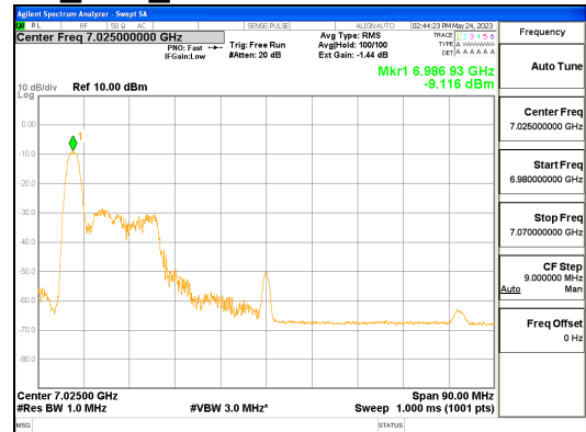
ANT L_802.11ax_HE80_26T_Low_UNII 8
