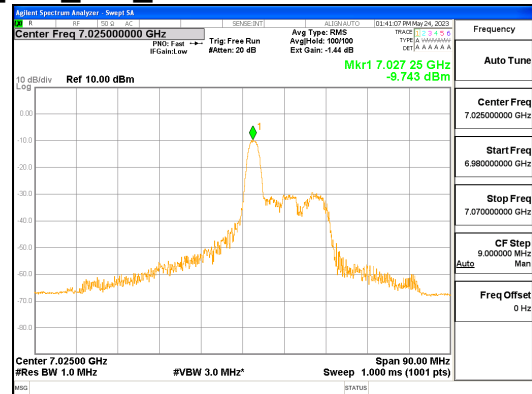
ANT R_802.11ax_HE80_26T_Mid_UNII 8
