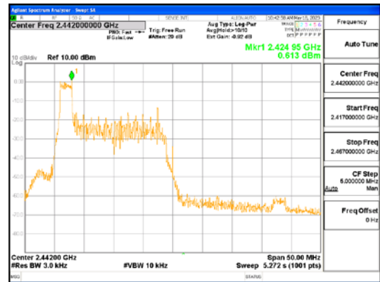
ANT L, 802.11ax_HE40_26T_Low
