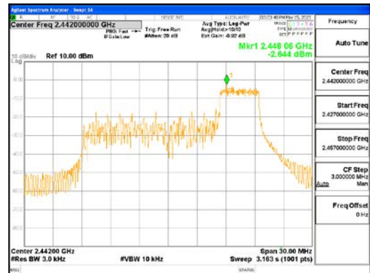
ANT L, 802.11ax_HE20_52T_High
