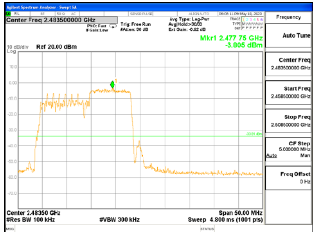
ANT L, 802.11ax_HE20_106T_High
