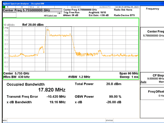
ANT R_802.11ax_HE40_26T_Low_UNII 3
