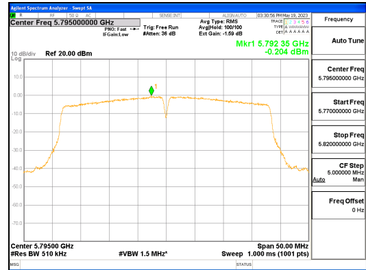
ANT R_802.11n_HT40_UNII 3
