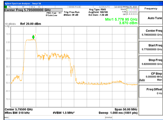
ANT L_802.11ax_HE40_52T_Low_UNII 3
