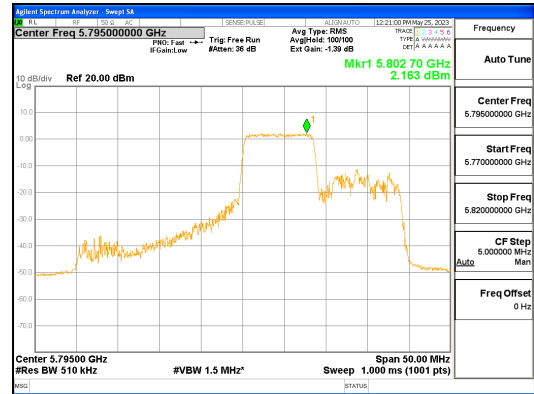
ANT L_802.11ax_HE40_106T_Mid_UNII 3
