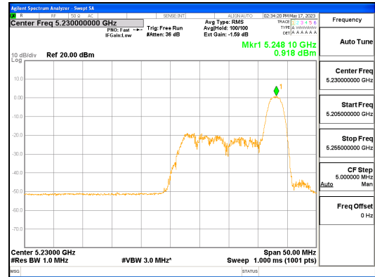
ANT R_802.11ax_HE40_26T_High_UNII 1
