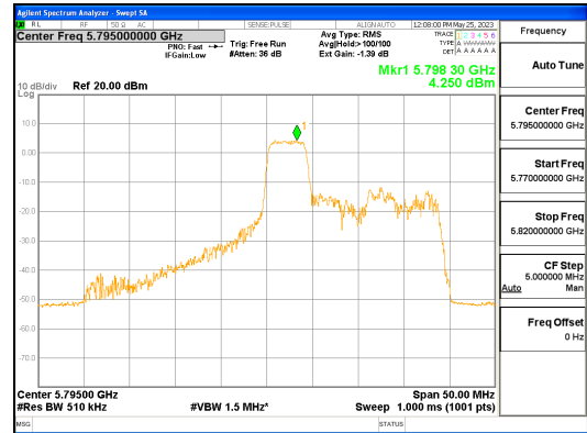
ANT L_802.11ax_HE40_52T_Mid_UNII 3
