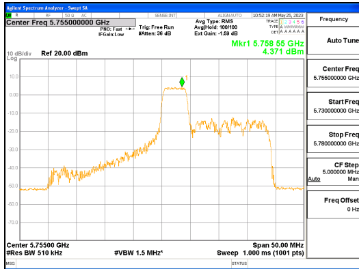
ANT R_802.11ax_HE40_52T_Mid_UNII 3
