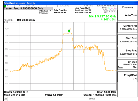
ANT R_802.11ax_HE40_52T_Mid_UNII 3
