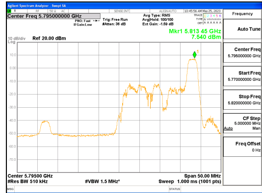
ANT R_802.11ax_HE40_26T_High_UNII 3
