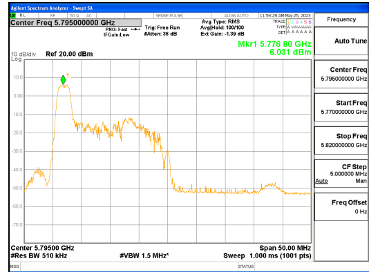
ANT L_802.11ax_HE40_26T_Low_UNII 3
