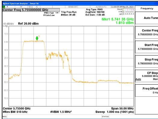
ANT R_802.11ax_HE40_106T_Low_UNII 3
