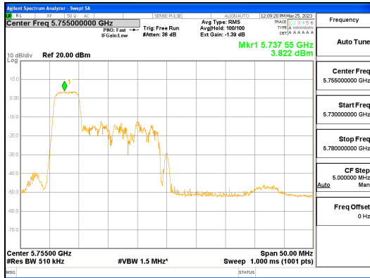
ANT L_802.11ax_HE40_52T_Low_UNII 3
