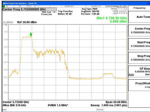
ANT R_802.11ax_HE40_52T_Low_UNII 3
