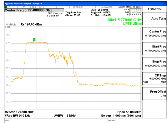
ANT R_802.11ax_HE40_106T_Low_UNII 3
