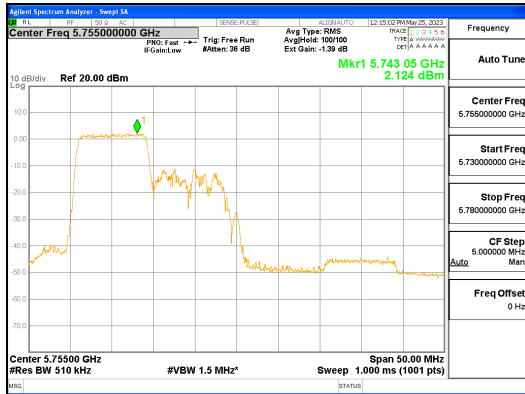
ANT L_802.11ax_HE40_106T_Low_UNII 3
