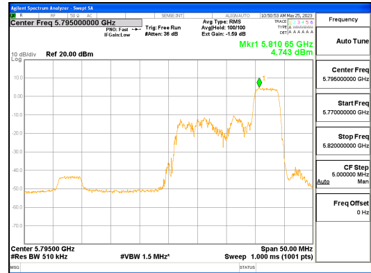
ANT R_802.11ax_HE40_52T_High_UNII 3
