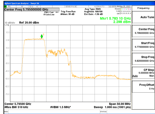
ANT L_802.11ax_HE40_106T_Low_UNII 3
