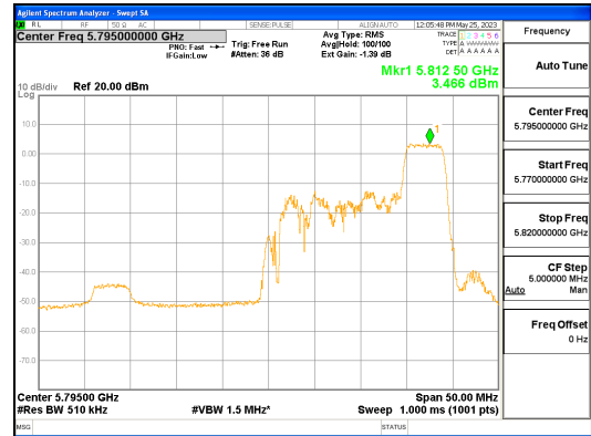
ANT L_802.11ax_HE40_52T_High_UNII 3
