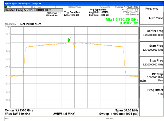
ANT L_802.11ax_HE40_484T_UNII 3
