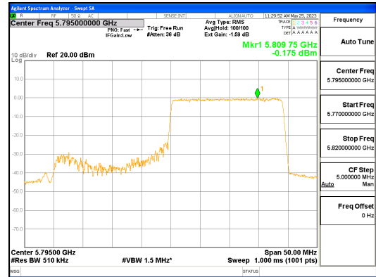
ANT_R_802.11ax_HE40_242T_High_UNII 3
