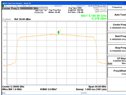
ANT R_802.11ax_HE40_484T_UNII 1
