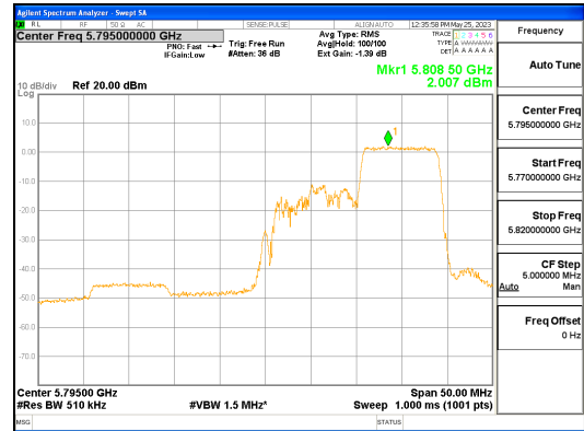
ANT L_802.11ax_HE40_106T_High_UNII 3
