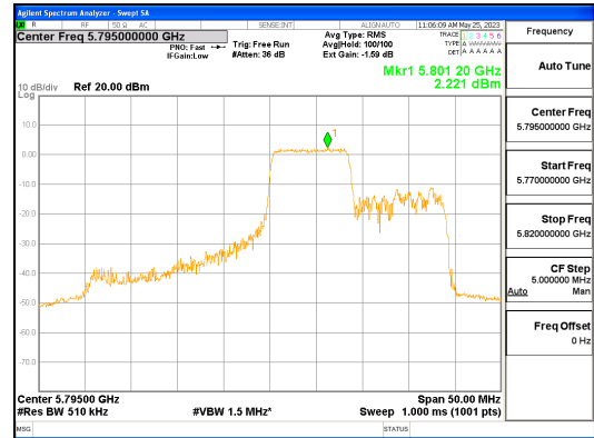
ANT R_802.11ax_HE40_106T_Mid_UNII 3
