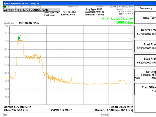
ANT R_802.11ax_HE80_52T_Low_UNII 3
