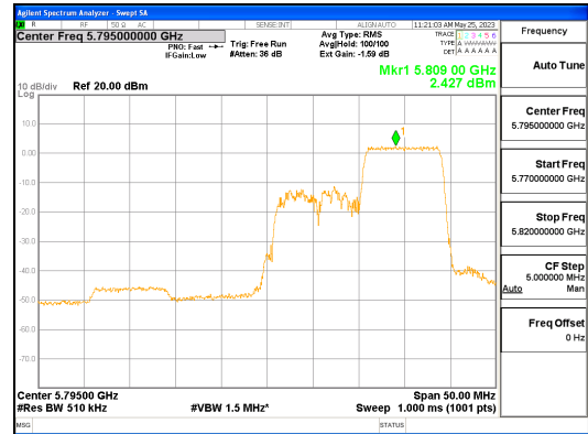
ANT_R_802.11ax_HE40_106T_High_UNII 3
