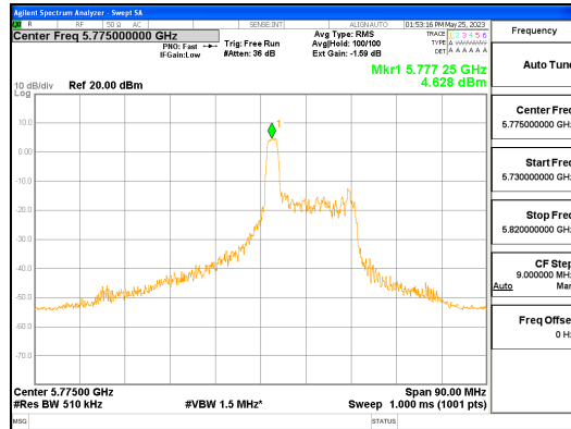
ANT R_802.11ax_HE80_26T_Mid_UNII 3
