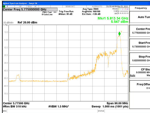
ANT R_802.11ax_HE80_26T_High_UNII 3
