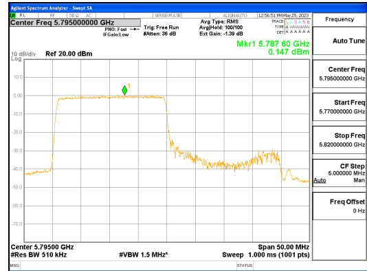
ANT L_802.11ax_HE40_242T_Low_UNII 3
