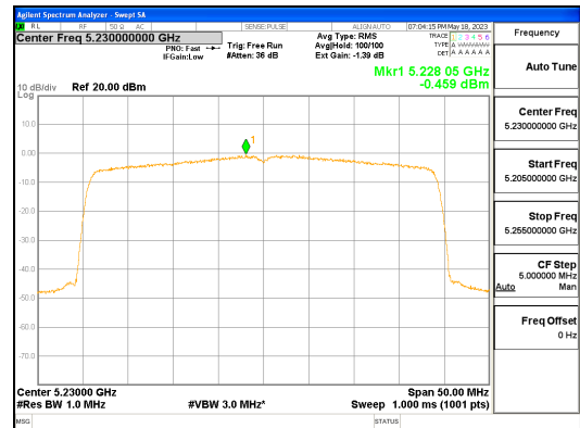
ANT L_802.11ax_HE40_484T_UNII 1
