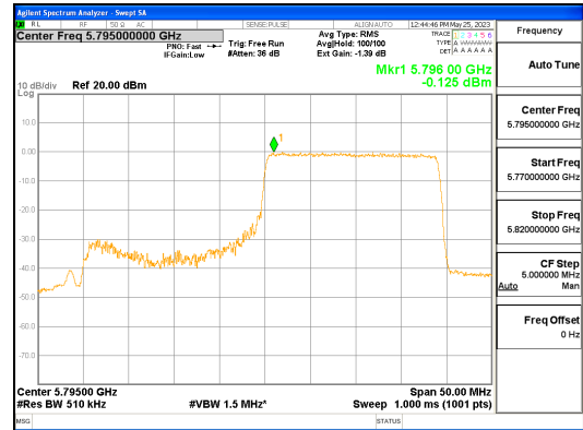
ANT L_802.11ax_HE40_242T_High_UNII 3
