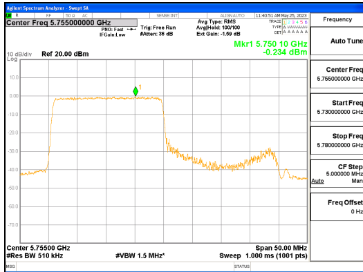
ANT R_802.11ax_HE40_242T_Low_UNII 3
