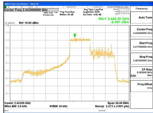
ANT0, 802.11ax_HE40_106T_Mid
