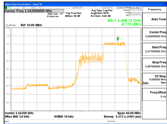
ANT0, 802.11ax_HE40_106T_High
