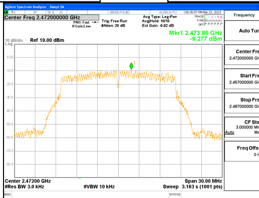
ANT0, 802.11g
