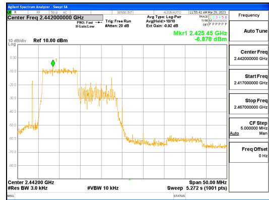
ANT0, 802.11ax_HE40_106T_Low
