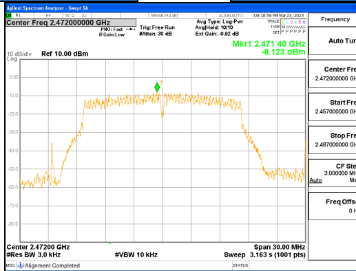
ANT1, 802.11g
