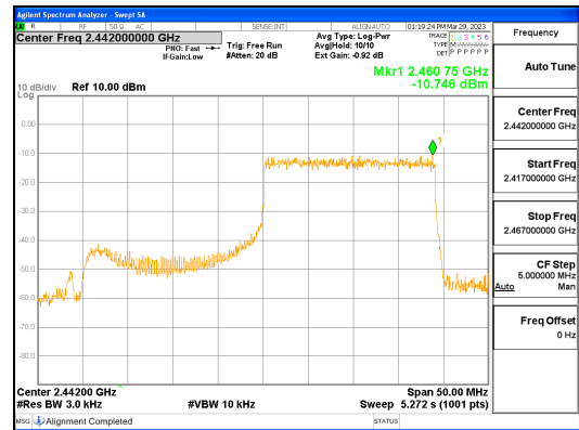
ANTO, 802.11ax_HE40_242T_High
