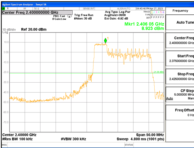
ANT1, 802.11ax_HE20_52T_Low
