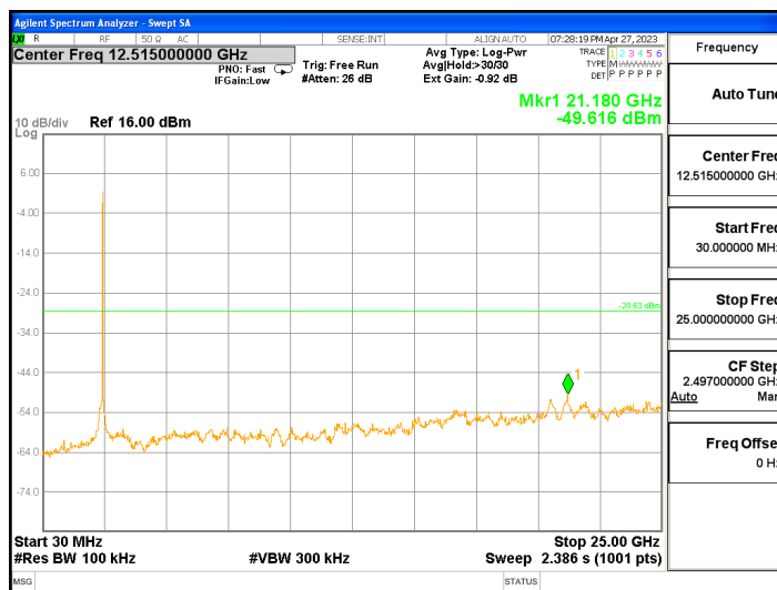
ANT1, 802.11ax_HE20_242T
