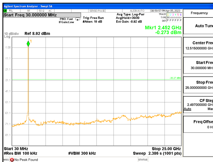
ANTO, 802.11ax_HE20_26T_Low
