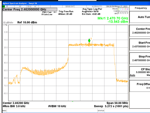
ANT1, 802.11ax_HE40_242T_High
