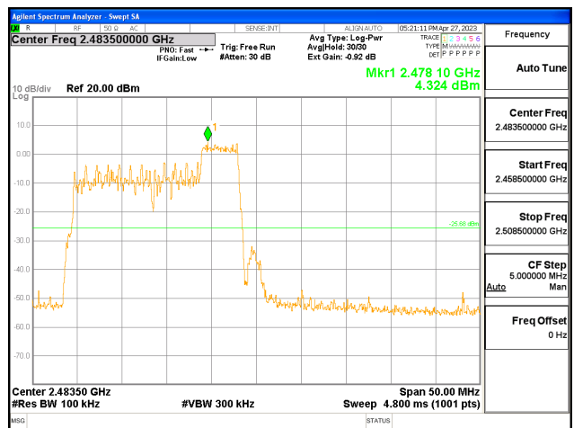
ANT1, 802.11ax_HE20_52T_High
