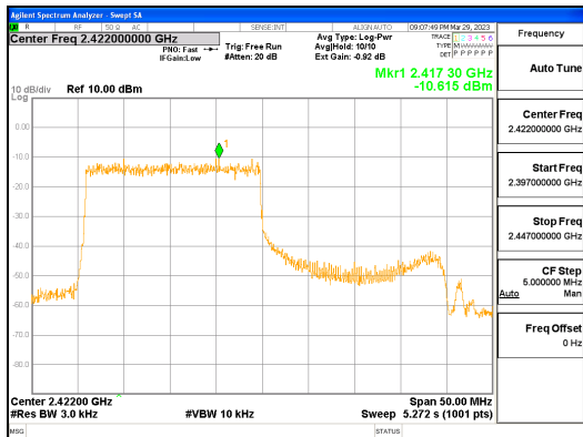
ANT0, 802.11ax_HE40_242T_Low
