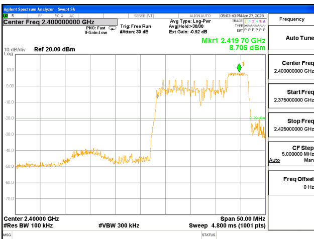
ANT1, 802.11ax_HE20_52T_High
