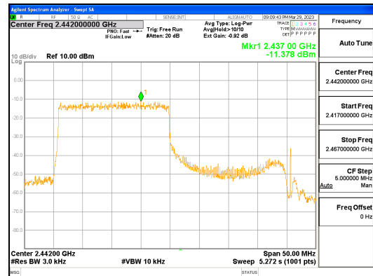
ANT0, 802.11ax_HE40_242T_Low
