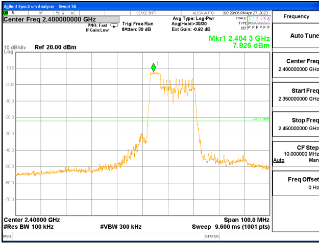
ANT1, 802.11ax_HE40_52T_Low
