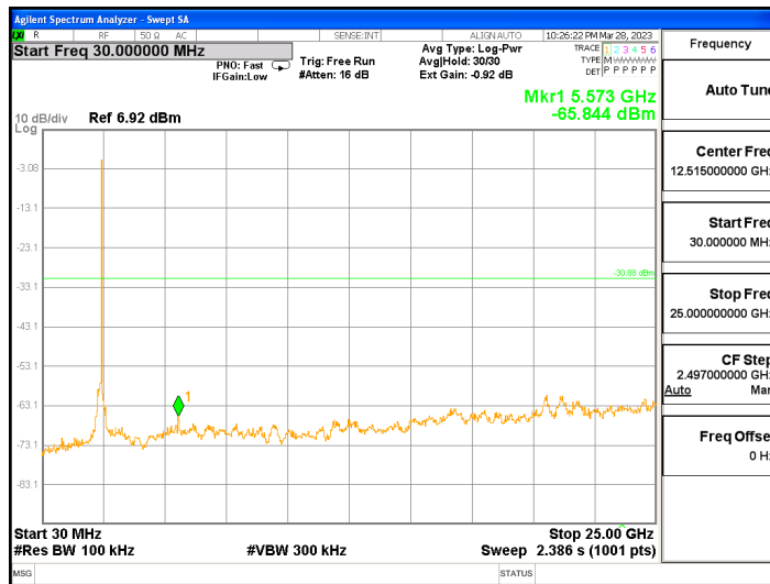
ANT1, 802.11ax_HE40_26T_Mid
