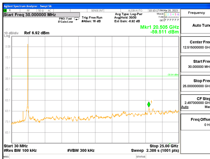
ANT1, 802.11ax_HE40_26T_Low
