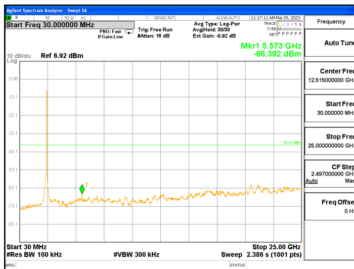
ANT1, 802.11ax_HE40_484T
