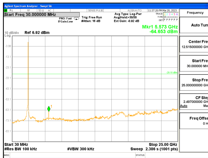
ANT0, 802.11ax_HE40_26T_Mid
