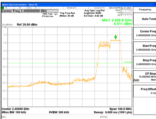
ANT1, 802.11ax_HE40_106T_High
