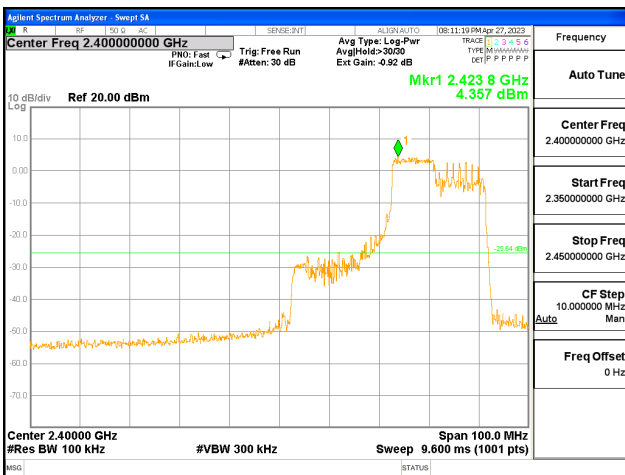
ANT1, 802.11ax_HE40_106T_Mid
