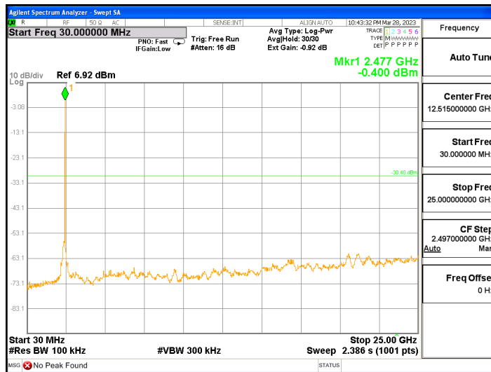
ANT1, 802.11ax_HE40_26T_High
