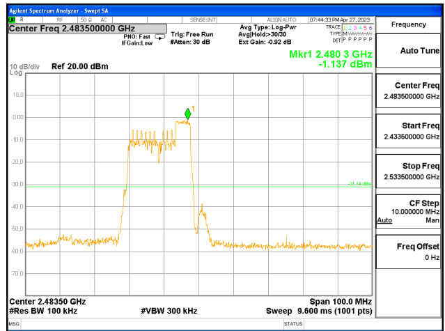
ANT1, 802.11ax_HE40_52T_High
