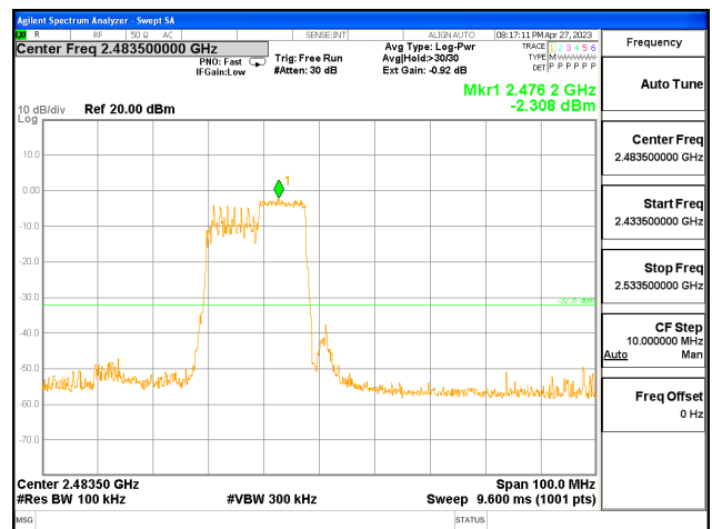
ANT1, 802.11ax_HE40_106T_High
