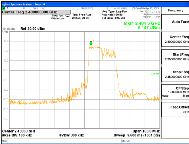
ANT1, 802.11ax_HE40_106T_Low
