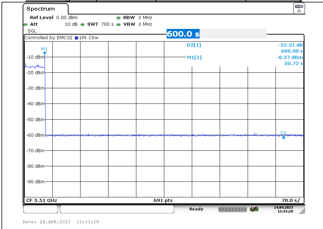
Monitoring live spectrum – Elapse time 10 minutes (40 MHz BW)
