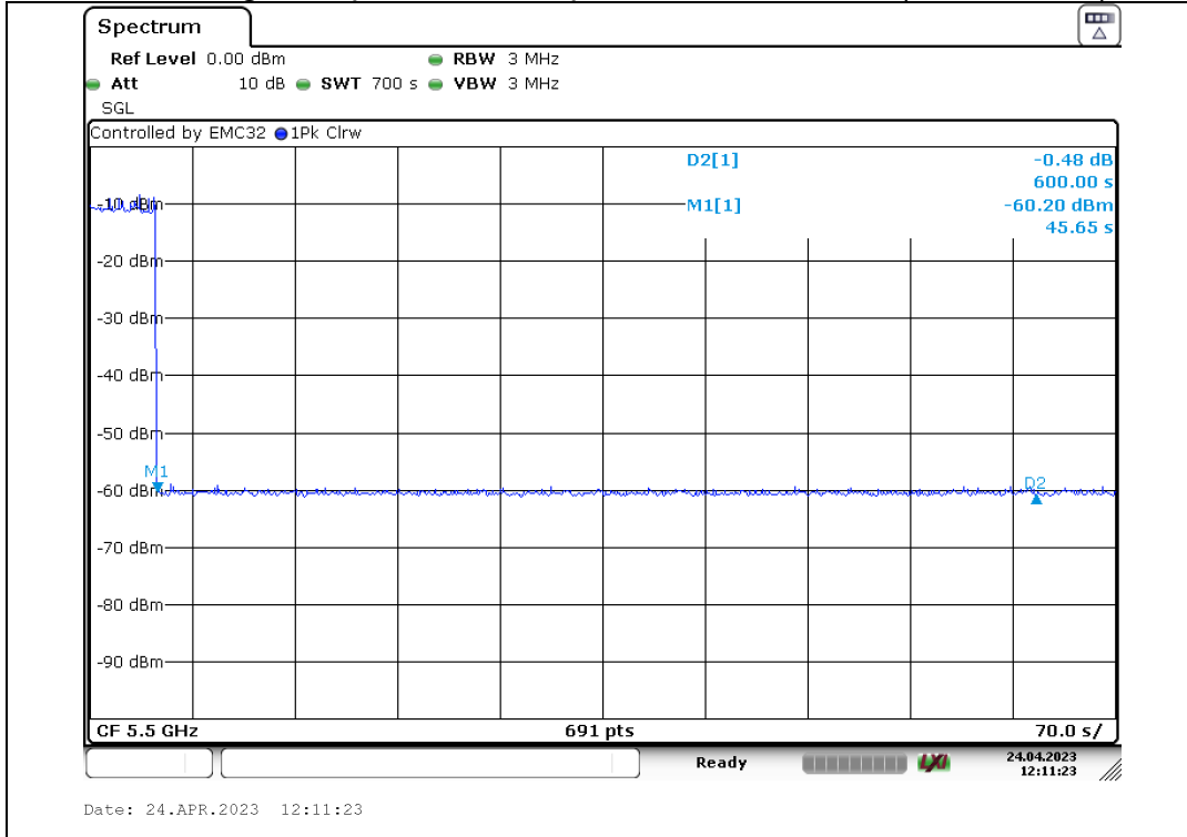
Monitoring live spectrum – Elapse time 10 minutes (20 MHz BW)
