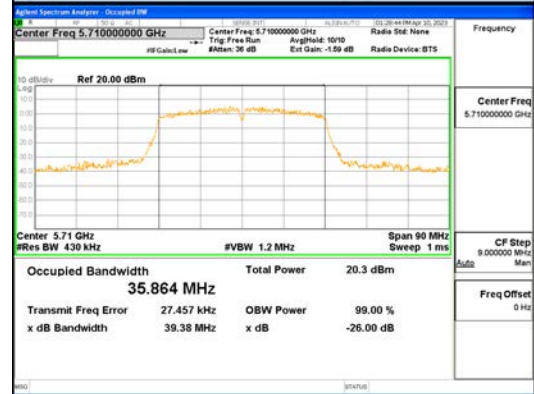
ANT1_802.11n_HT40_UNI I 2C
