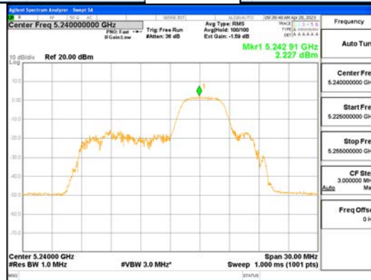
ANT1_802.11ax_HE20_52T_Mid_UNI1 1
