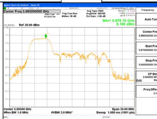
ANT1_802.11ax_HE20_52T_Low_UNI I 4
