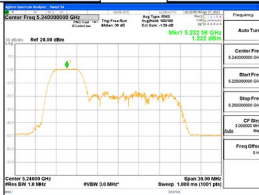
ANT1_802.11ax_HE20_52T_Low_UNI 1
